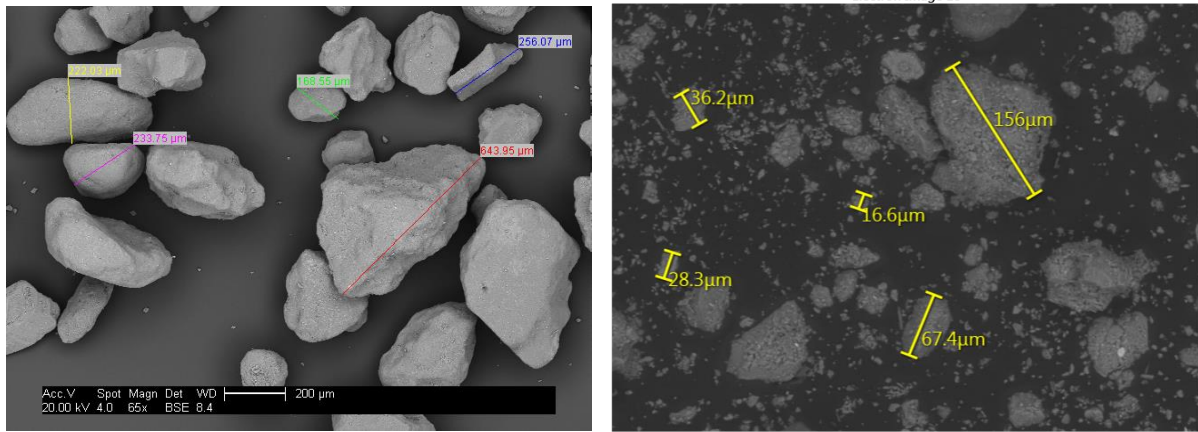
FIGURE 4a. Particles collected at ground level (Iran)
