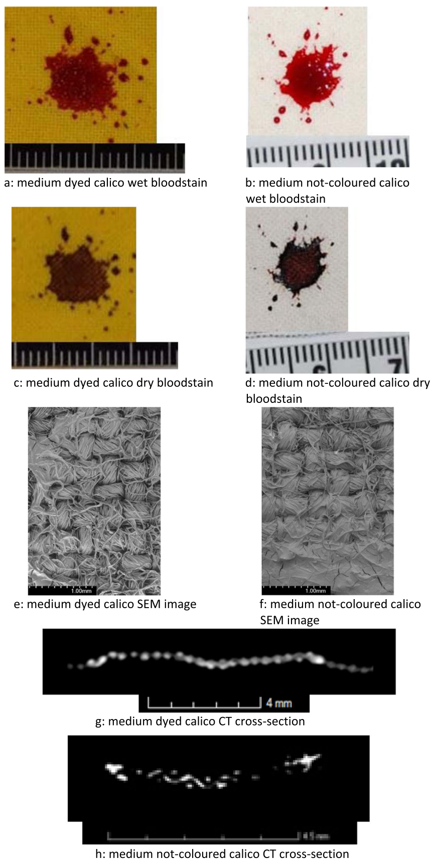
Fig. 11. examples of wet and dry bloodstain photograph (scale: 2 cm), SEM image at 42x magnification and CT cross-section in the weft direction on the medium dyed and not-coloured calico (images taken for research [10] but not used in publication) from 4.1 \text{ ms}^{-1} .
