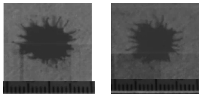
a: not-coloured, area 104 \text{ mm}^2 b: dyed, area 103 \text{ mm}^2
