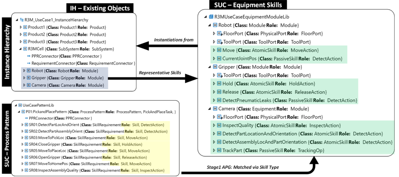
Fig. 18. Overview of Equipment, its Skills, and Process Pattern
