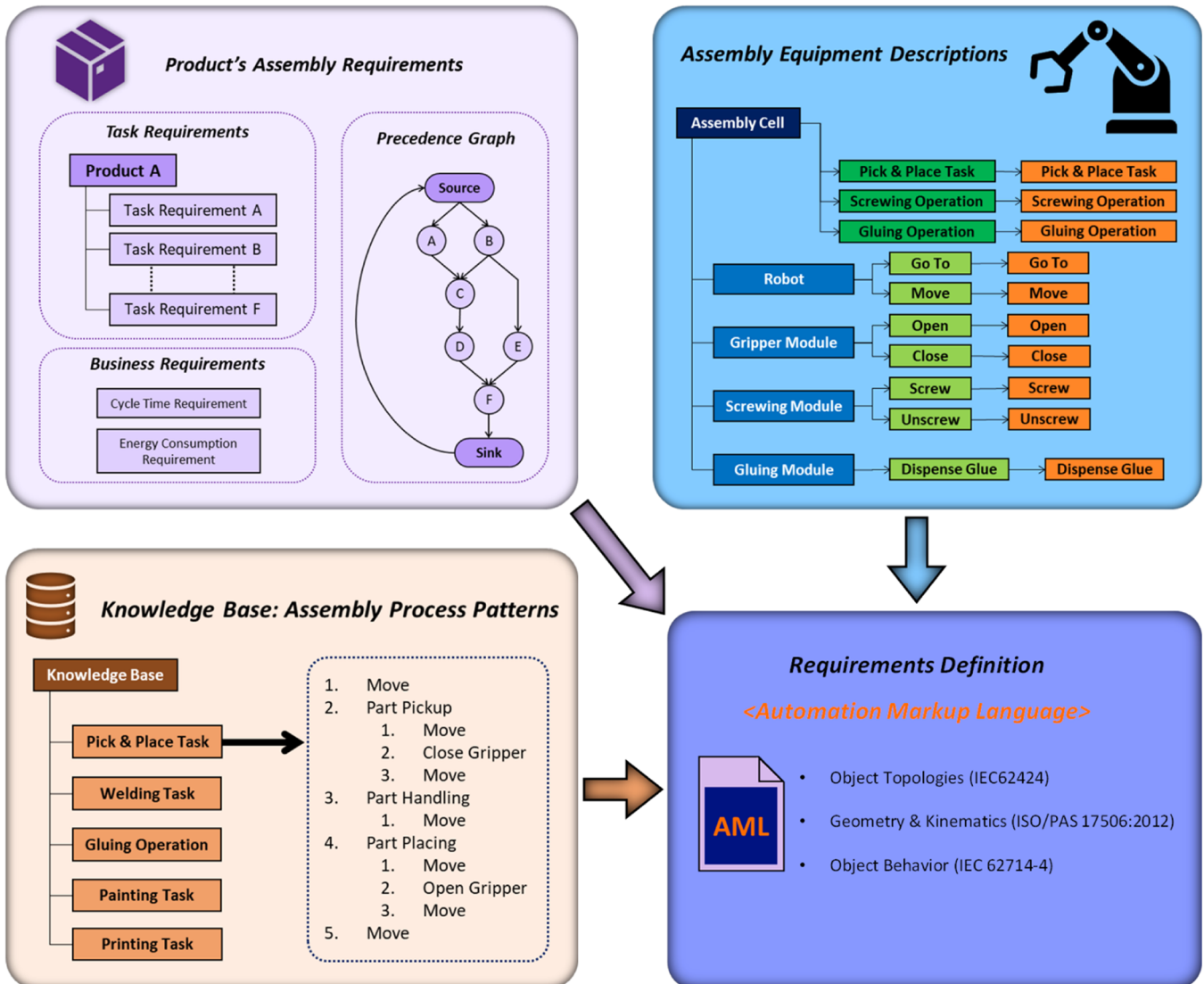
Fig. 6. Overview of Requirements Definition
