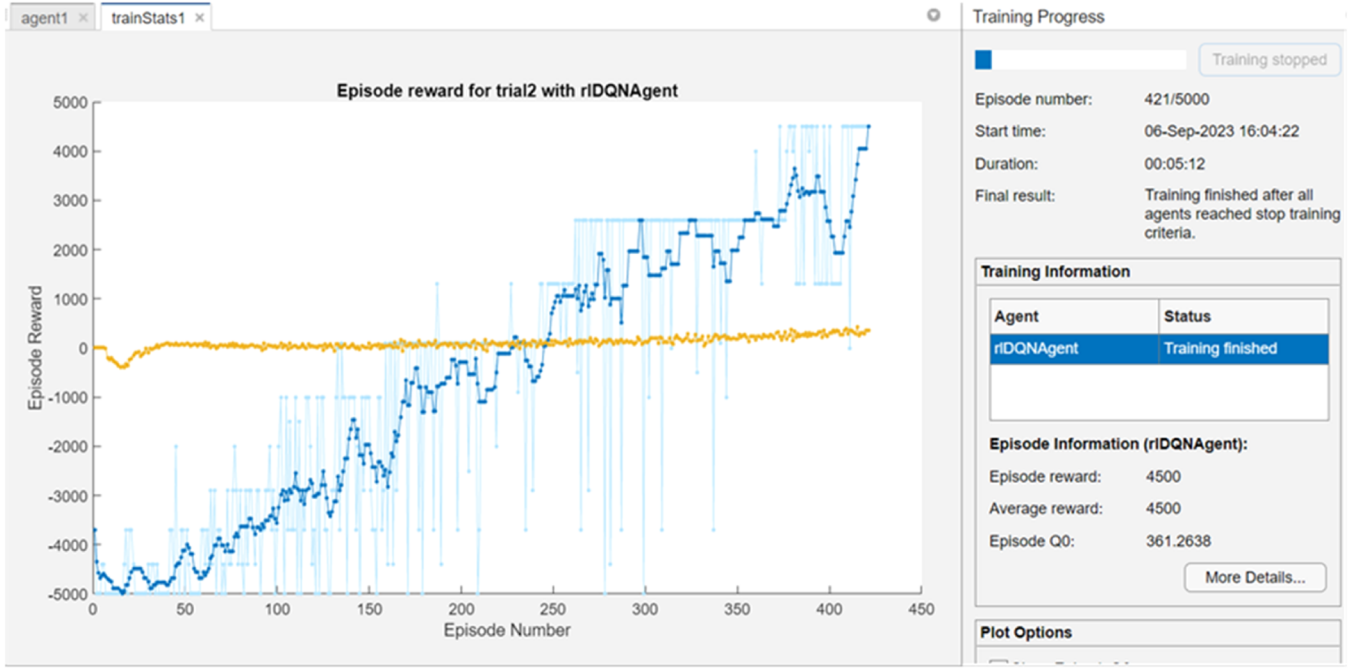
Fig. 20. Overview of the Progress of the RL Training Episodes
