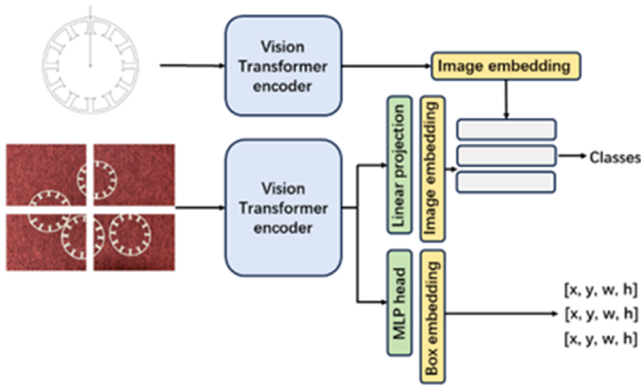
Fig. 12. OWL-ViT architecture
