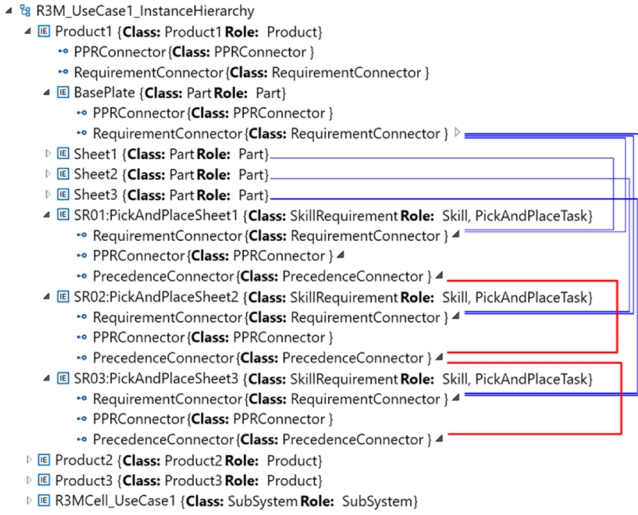
Fig. 17. Use-Case's Product Definition in AML
