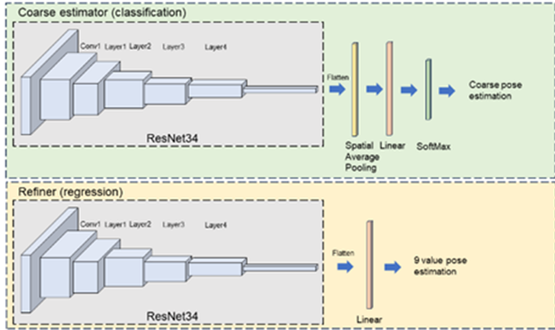
Fig. 14. Computational Models of MegaPose
