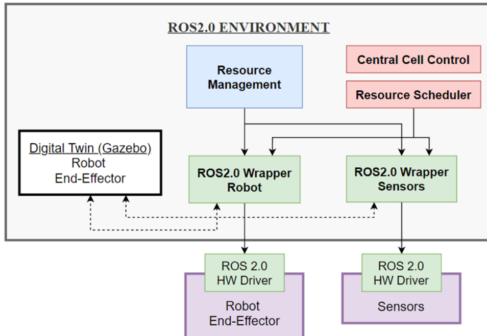
Fig. 5. Simplified Architecture of the R3M-ROS2 Environment
