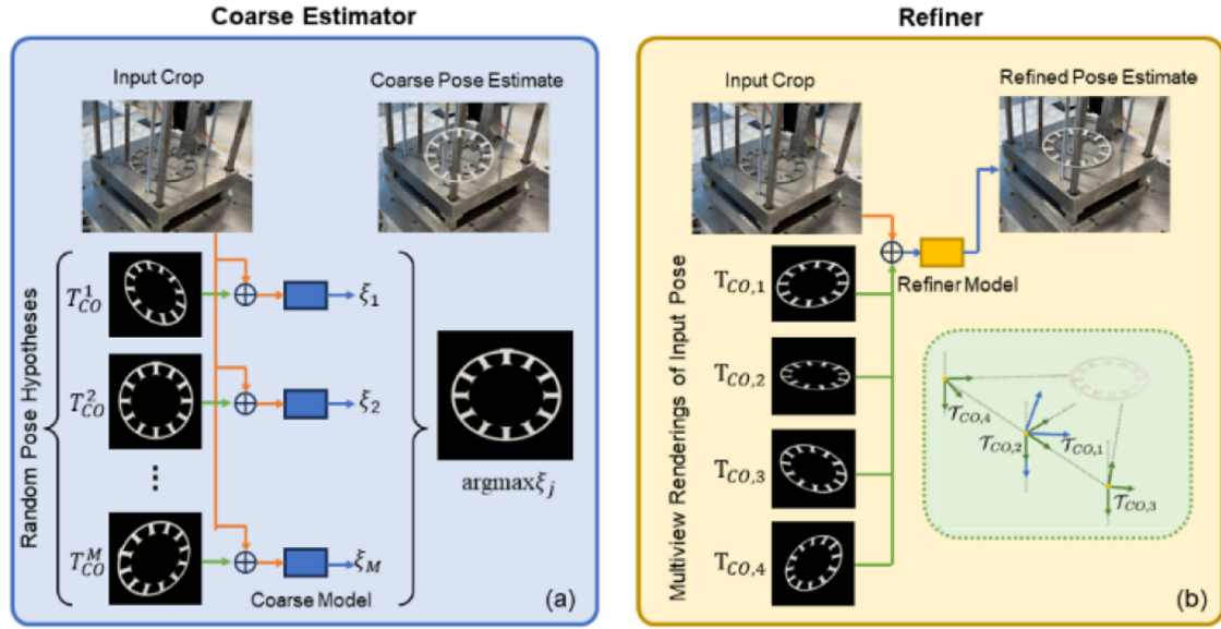
Fig. 13. MegaPose Architecture
