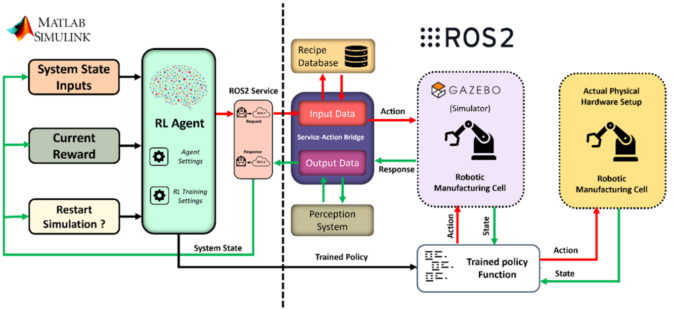
Fig. 10. Overview of RL Setup and ROS2-based Skill Execution
