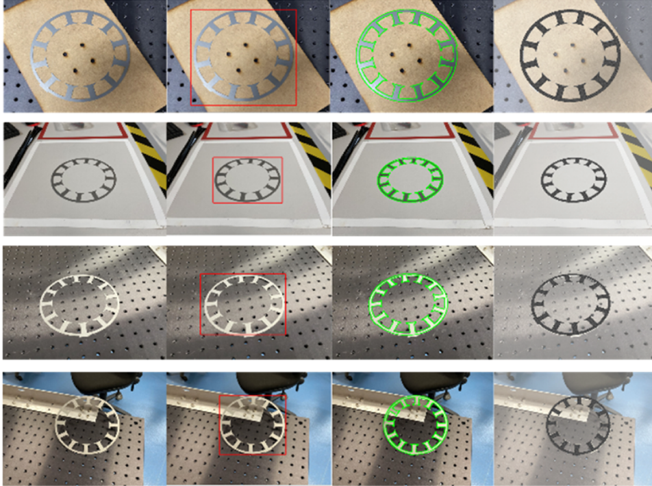
Fig. 21. (a) Camera observations, (b) Results of novel object detection, (c) Contour overlay rendered from estimated 6DoF pose, (d) Mesh overlay rendered from 6DoF pose.
