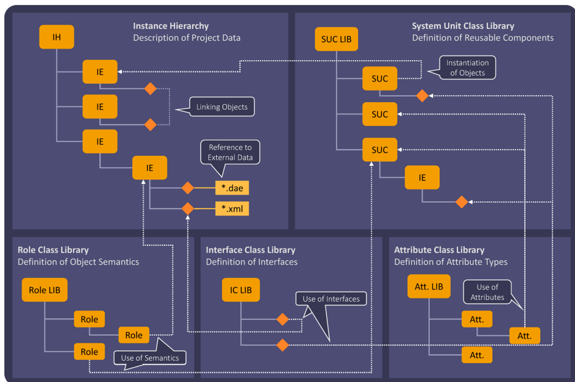
Fig. 8. Overview of the AML Class Libraries and its uses
