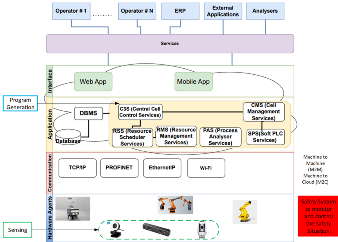
Fig. 4. R3M Software Architecture
