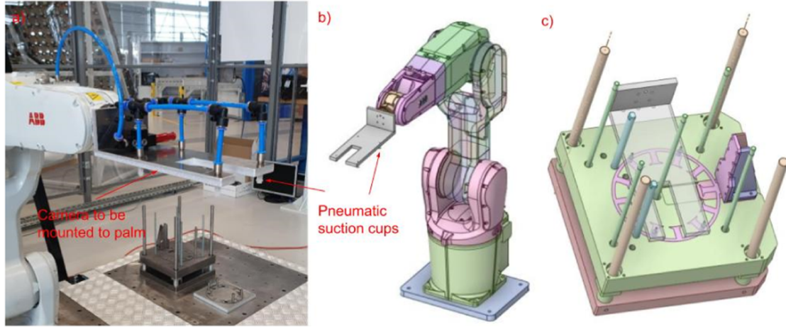
Fig. 16. (a) Image of the designed end effector on an ABB IRB 1200 robot with pneumatic suction cups for the lamination stacking application, (b) CAD model of the end effector and (c) CAD model showing the end effector passing over the fixture to place the sheet.
