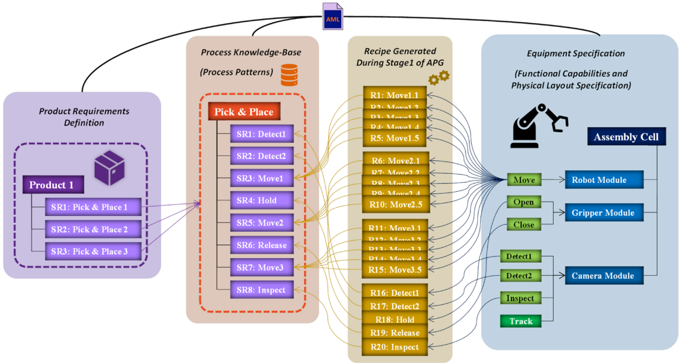
Fig. 19. Overview of the Use-Case specific Product Requirements and Equipment Skills
