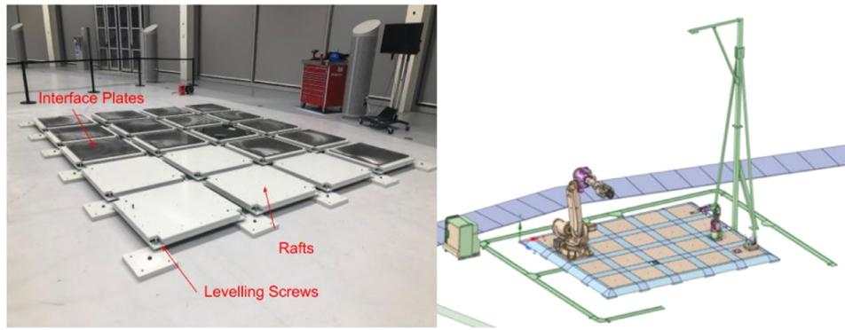
Fig. 2. Reconfigurable Cell Demonstrator. (left) Image of RECON Cell's reconfigurable floor during assembly. (right) CAD model of current RECON Cell containing a large ABB IRB-6640 robot, a small ABB IRB-1200 robot and a tall mounting fixture for sensors.
