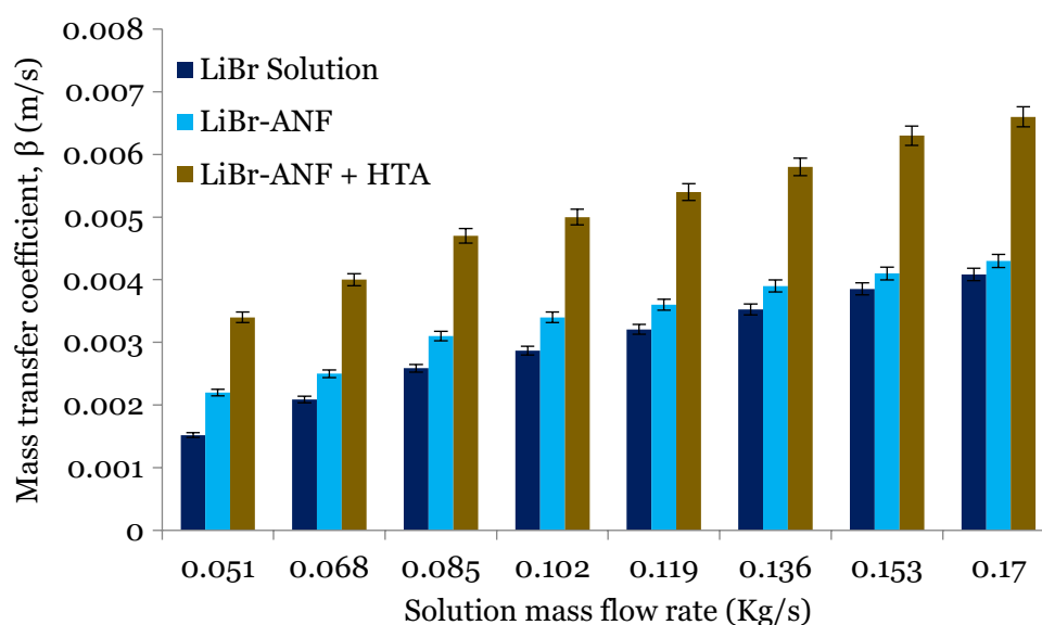
Fig. 7 Nanofluid testing: mass transfer coefficient against solution mass flowrate
