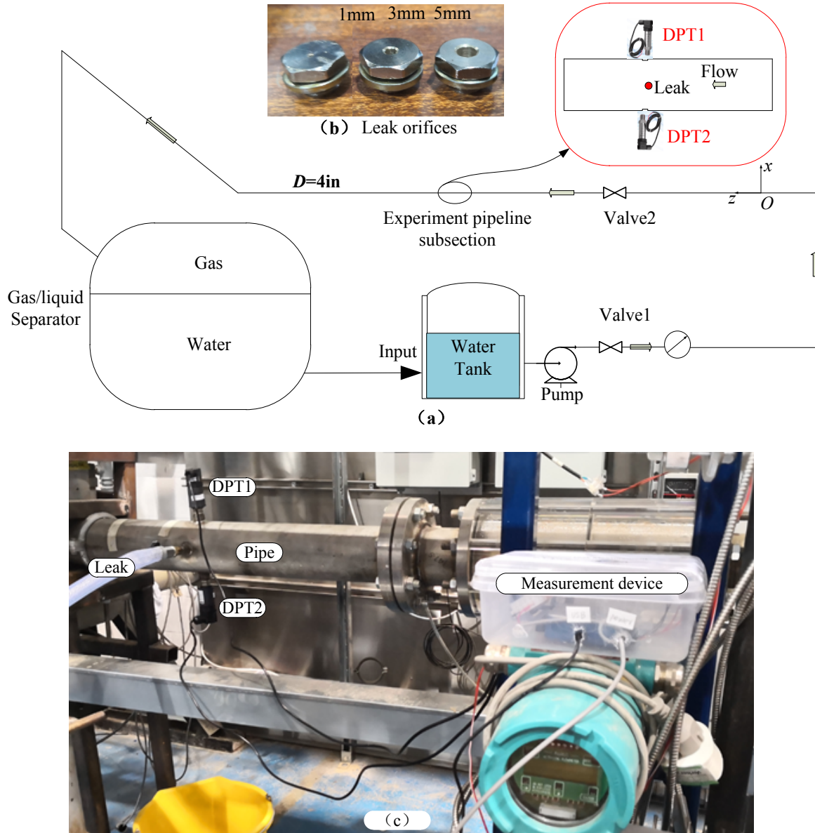
Fig.2 Experimental platform loop. (a) Schematic; (b) Leak orifices; (c) Experimental pipeline subsection.
