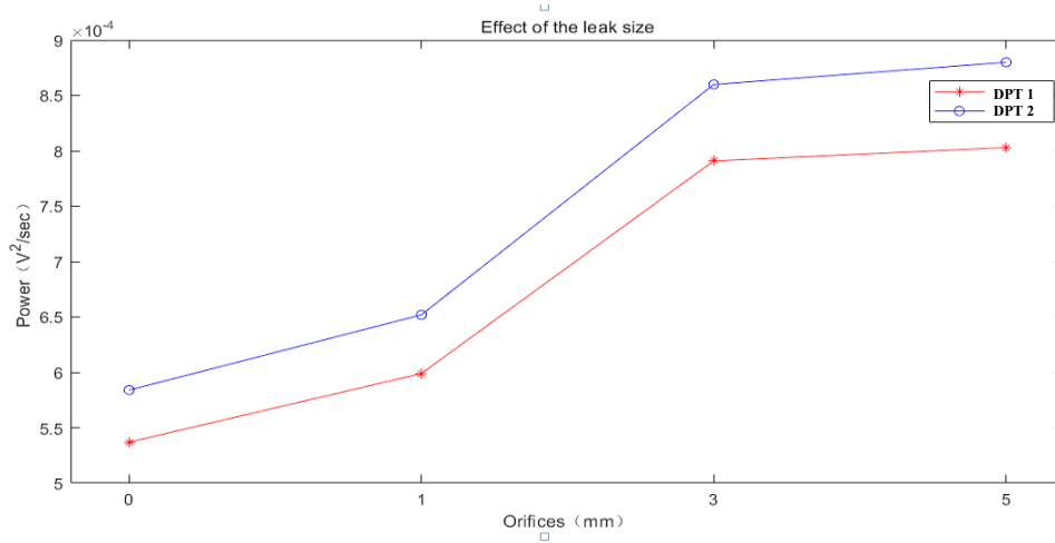
Fig.6 signal intensity against the leak size.
