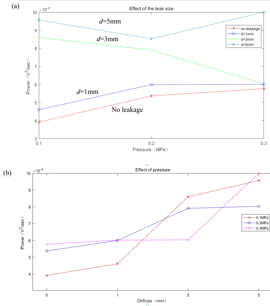
Fig.7 Effects of pipeline pressure. (a) Signal intensity against the pressure; (b) Power of DPT 1 in different pipeline pressure.
