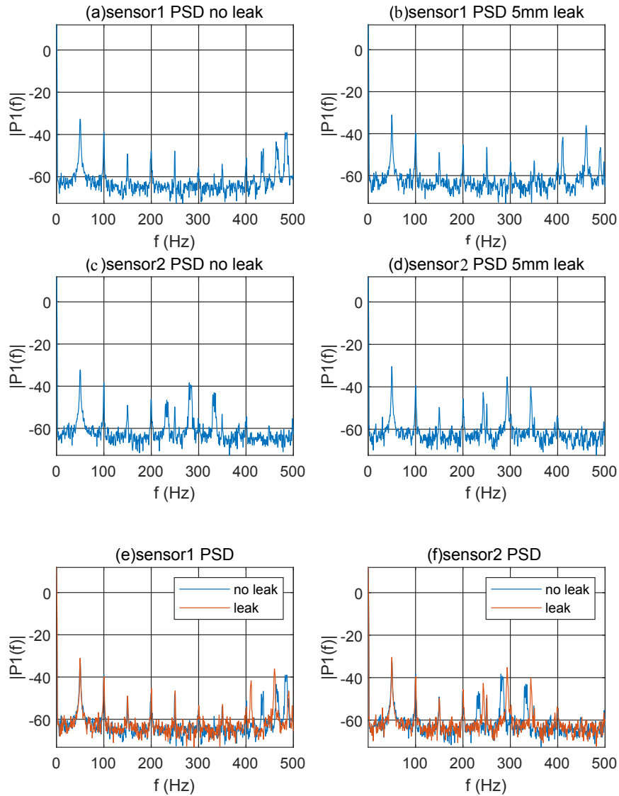
Fig.5 PSD of two DPTs (0.2MPa, 5mm, 1m/s): (a) DPT 1, no leak; (b) DPT 1, leak; (c) DPT 2, no leak; (d) DPT 2, leak; (e) DPT 1, comparison; (f) DPT 2, comparison.
