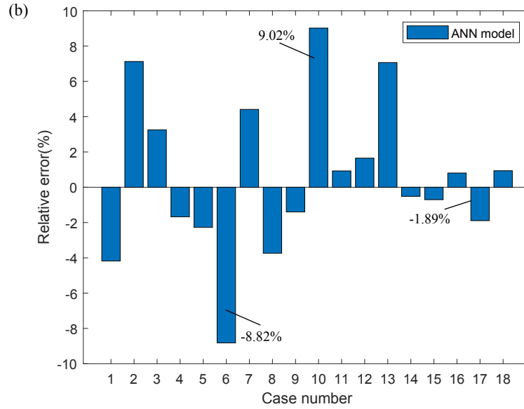
Fig. 11 Comparison of the leak diameter obtained by experiment and ANN model. (a) the prediction results;(b) the relative error.
