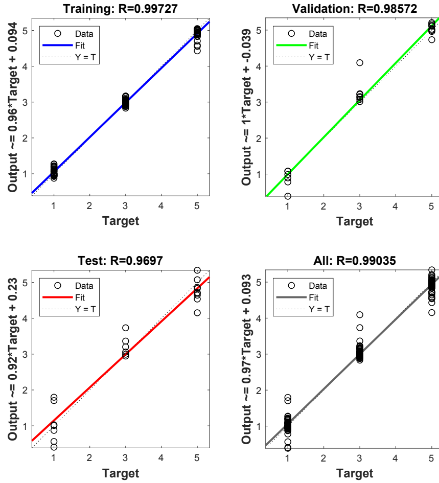
Fig. 10 Neural network target to output fitting curve.
