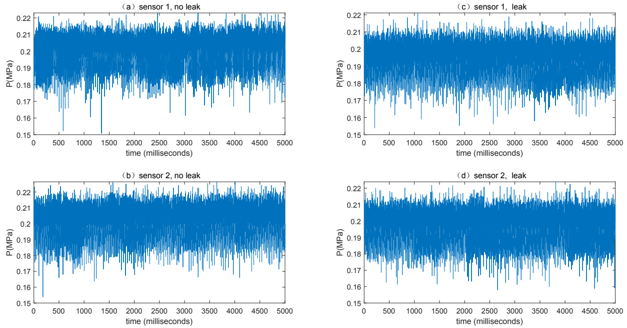
Fig. 3 Dynamic pressure of two DPTs (0.20MPa, 5mm, 1m/s) : (a)DPT 1, no leak; (b)DPT 2, no leak; (c)DPT 1, 5mm leak; (d)DPT 2, 5mm leak.
