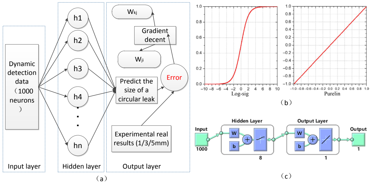
Fig. 9 Artificial neural network. (a) structure for leak detection; (b) activation functions; (c) neural network.
