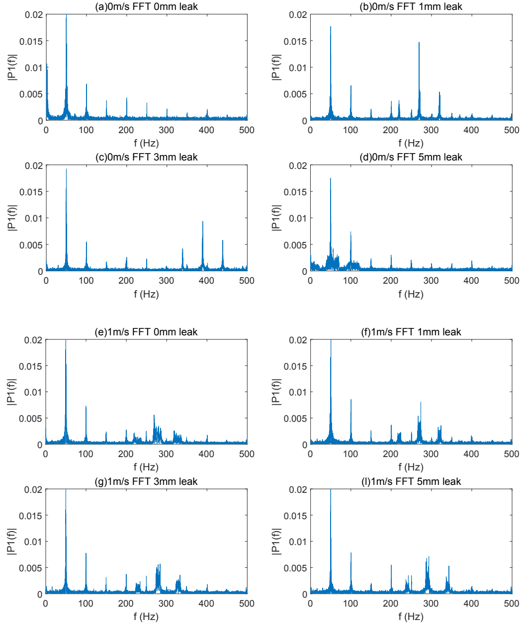
Fig. 15 DPT2, FFT (0.20MPa). (a) 0m/s, no leak; (b) 0m/s, 1mm; (c) 0m/s, 3mm; (d) 0m/s, 5mm; (e) 1m/s, no leak; (f) 1m/s, 1mm; (g) 1m/s, 3mm; (h) 1m/s, 5mm.
