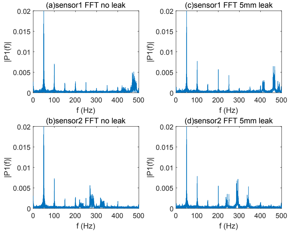
Fig. 4 FFT results of two DPTs' (0.20MPa, 5mm, 1m/s): (a)DPT 1, no leak; (b) DPT 2, no leak; (c) DPT 1, 5mm leak; (d) DPT 2, 5mm leak.
