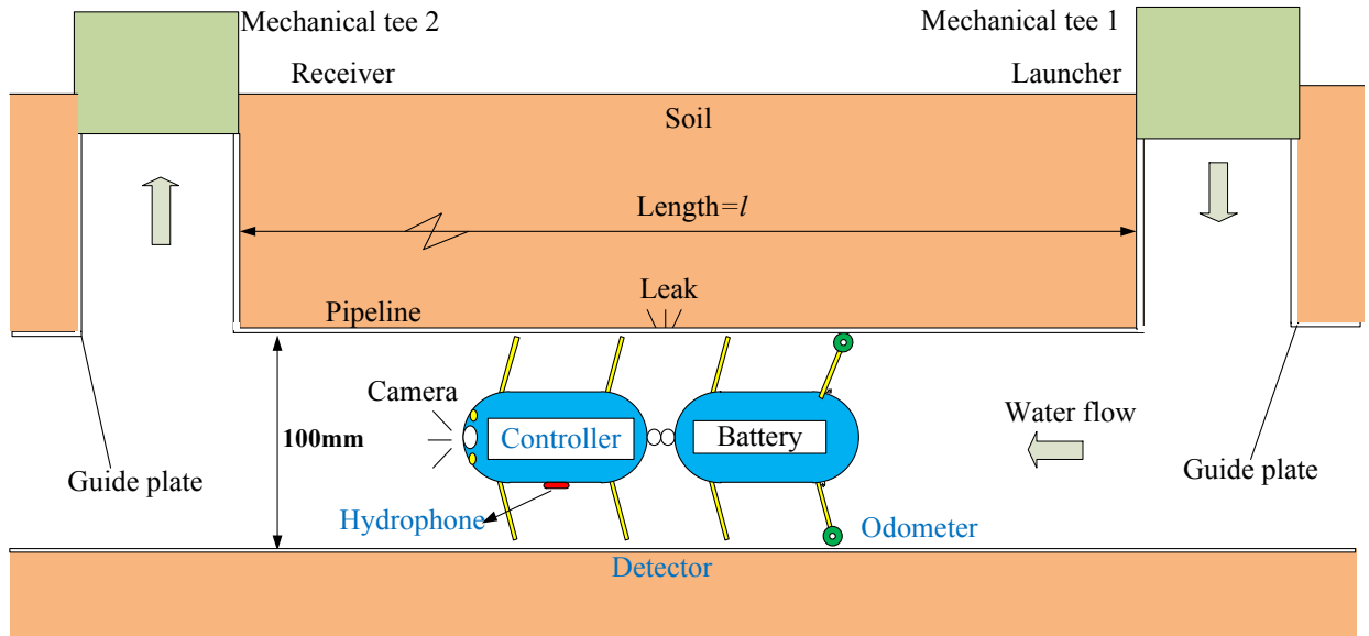
Fig.1 Scheme of the in-pipe detector.
