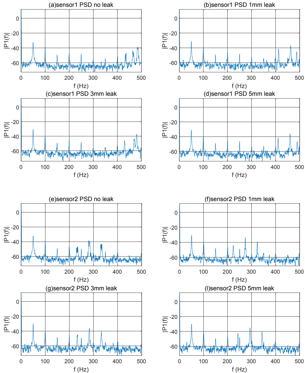
Fig. 13 DPT 1 and DPT 2, PSD (0.20MPa, 1m/s). (a) DPT 1, no leak; (b) DPT 1, 1mm; (c) DPT 1, 3mm; (d) DPT 1, 5mm; (e) DPT 2, no leak; (f) DPT 2, 1mm; (g) DPT 2, 3mm; (h) DPT 2, 5mm.
