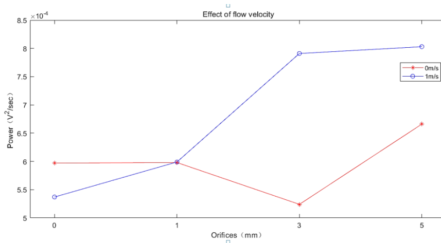
Fig.8 Signal intensity against the flow velocity.
