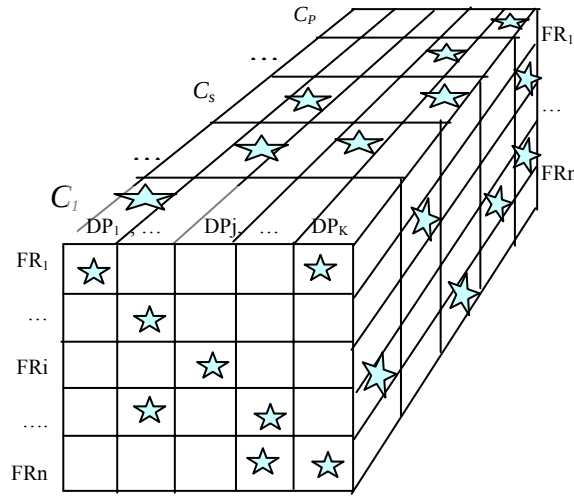
Fig.6. The design cube . Constraints (C) affect functional requirements (FR) and the choice and tolerances of the design parameters (DP).
