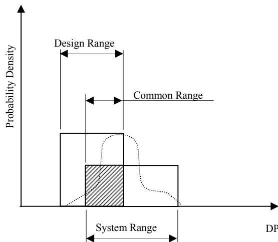
Fig. 3. Probability distribution of a design parameter. The solid line represents uniform distribution, the dotted line - a non-uniform distribution. (Adapted from Suh, 1990).
