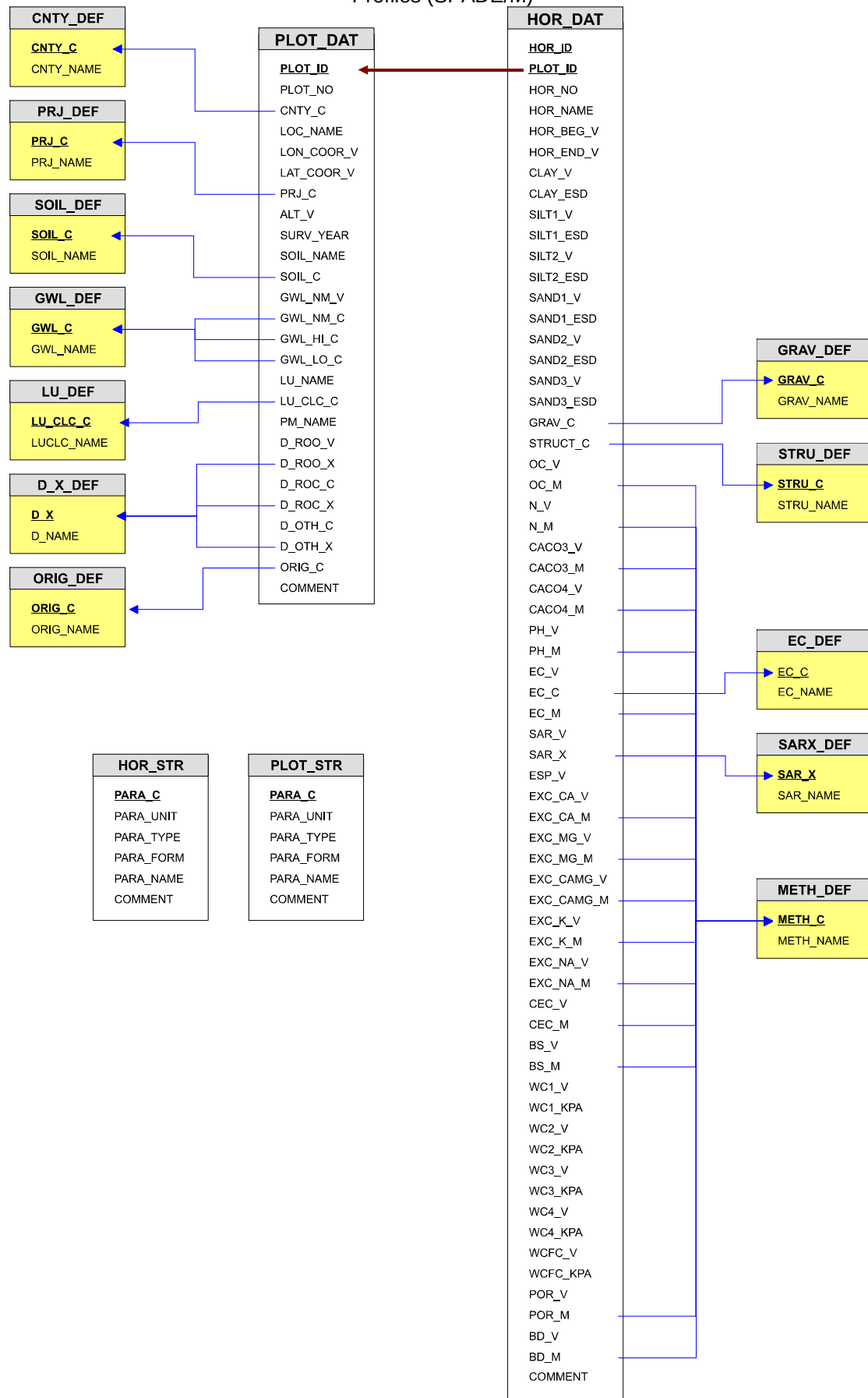
Figure 3 Schematic Data Model for Soil Profile Analytical Database of Europe of Measured Profiles (SPADE/M)
