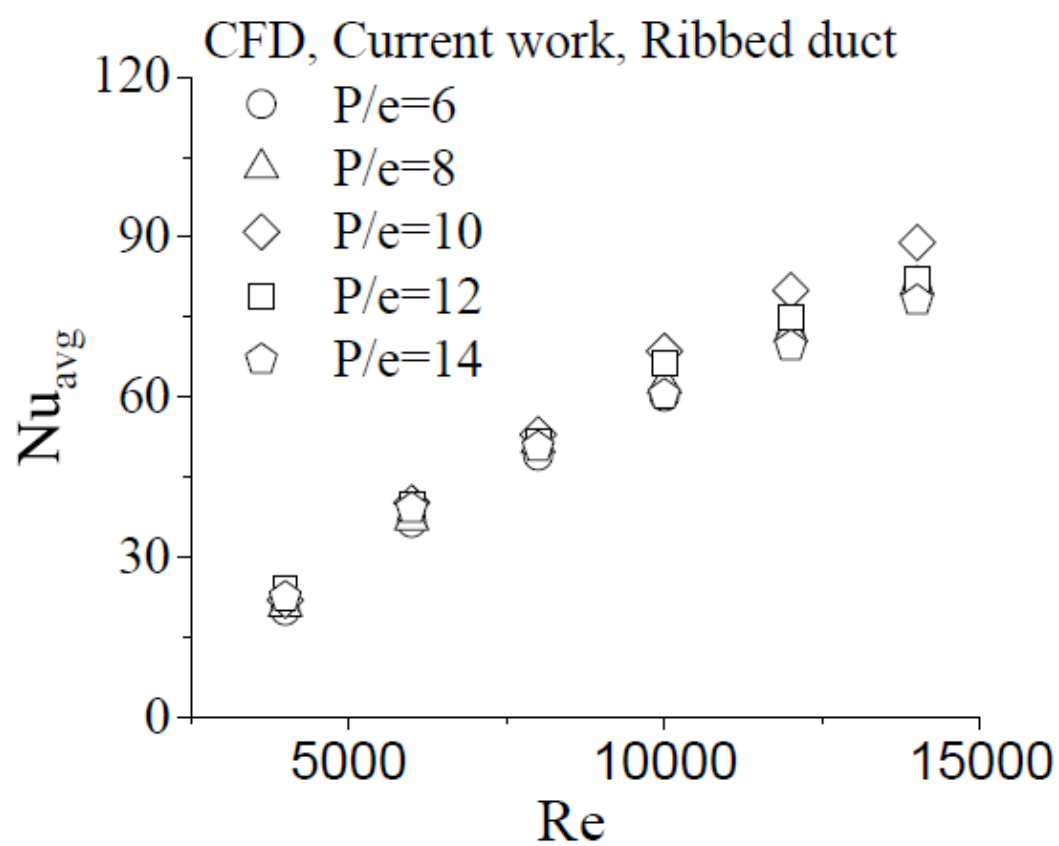
Figure 8: Comparison of averaged Nusselt numbers for different values of P/e
