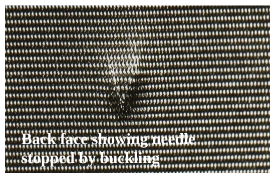
Figure 6. Puncture damage to lightweight metal mesh viewed under the microscope (x20)
