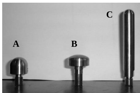
Figure 3. Tools used to determine impact forces
