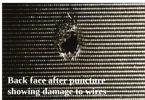
Figure 6. Puncture damage to lightweight metal mesh viewed under the microscope (x20)
