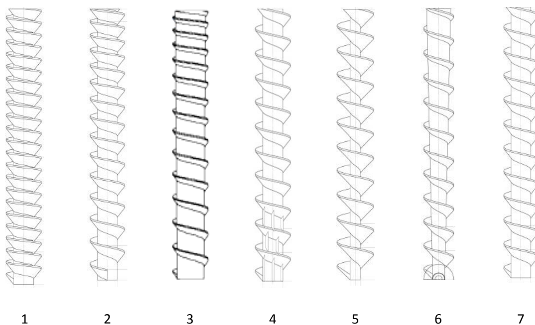
Figure 2. Schematics of screws 1-7.
