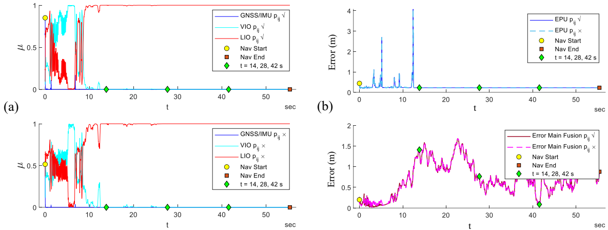
Figure 7. Results comparison with two different transition matrices, (a) showing the mixing weights and (b) the EPU and Main fusion error in meters.
