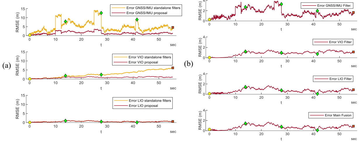
Figure 6. RMSE results, where (a) depicts a comparison between the error of standalone full-state Kalman independent filters for tracking the positioning signals and the full-state Kalman independent filters with the mixing process of the proposed architecture (see eq. (4)) while (b) shows the same three positioning signals from the proposed architecture with a fourth overall estimation composed of the associated weights for each signal (as seen in Figure 5.b)
