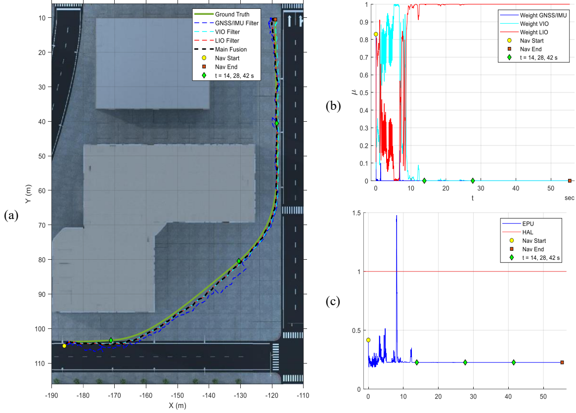
Figure 5. Proposed architecture results where (a) illustrate the overall estimation (black dotted line) and independent full-state Kalman filters (blue, cyan and red dotted lines). (b) shows the mixing weights for the independent filters and (c) the estimated position uncertainty of the overall estimation during the flight.
