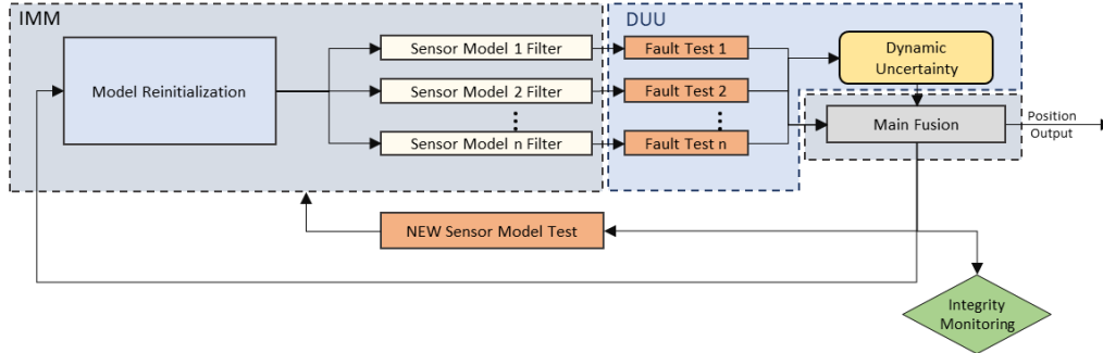
Figure 3. The system architecture of the proposed sensor fusion architecture with the state-of-the-art Dynamic Uncertainty Update (DUU) section. Every color represents different modules of the comprehensive architecture, while dashed lines represent the two main segments of the IMM adapted filter and DUU.
