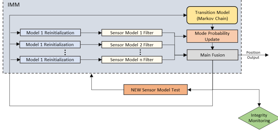
Figure 1. Resilient Interactive Sensor-Independent-Update Fusion methodology, an overview of the principal modules readapted from [4].
