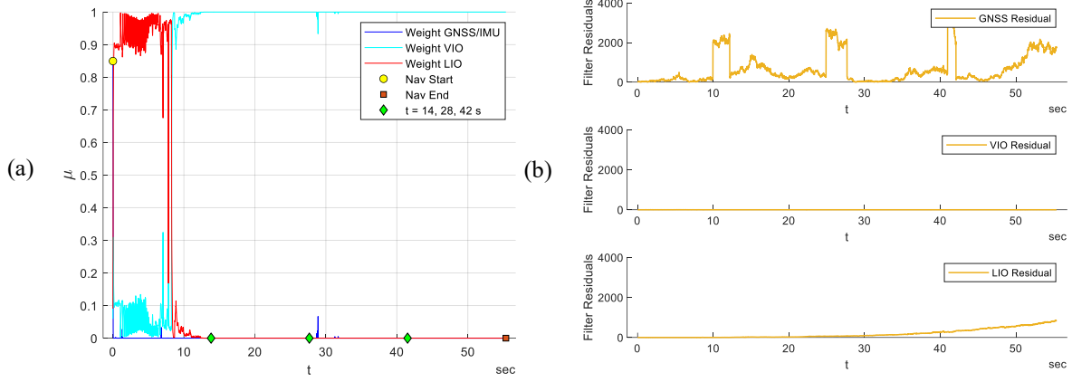
Figure 8. (a) Jump transition flow from LIO to VIO when a sudden change in the signal is presented. (b) shows the residuals of the independent filters, the value increases proportionally to the faults.
