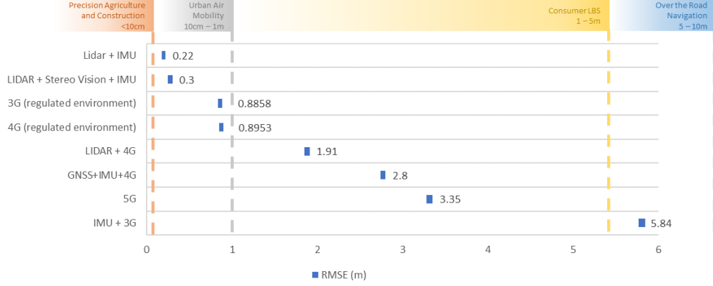
Figure 2. Comparison summary of recent positioning techniques for GNSS denied navigation [5]–[11]. For the convenience of the accuracy classification, the illustration adapts the standard developed in the report to congress from Homeland Security of the U.S. [12].
