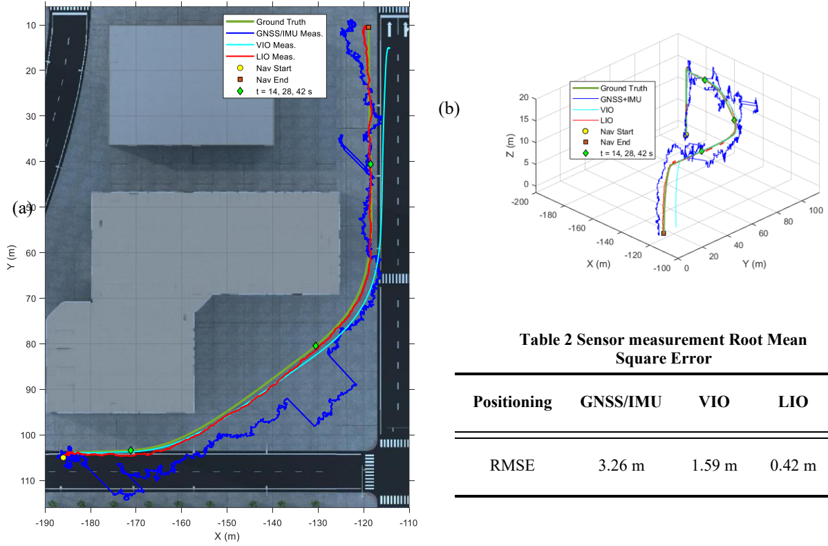
Figure 4. Simulation results for GNSS/IMU, VIO, and LIO position measurements. Control points are shown at the 25, 50 and 75% of the mission corresponding to 14, 28, and 42 seconds. a) shows the 2D projection of the measurements in the simulation environment, b) the three-dimensional measurements.
