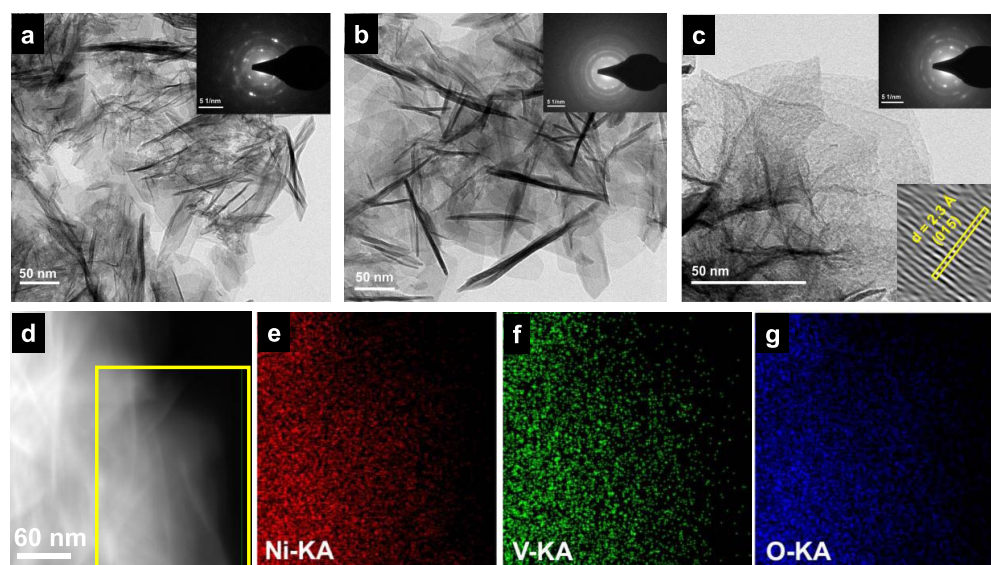
Figure 3. (a–c) TEM images of \text{Ni}_{0.67}\text{V}_{0.33} LDH, \text{Ni}_{0.75}\text{V}_{0.25} LDH, and \text{Ni}_{0.80}\text{V}_{0.20} LDH, respectively, and the insets show their corresponding SAED patterns, as well as the HRTEM image of \text{Ni}_{0.80}\text{V}_{0.20} LDH. (d) TEM image of \text{Ni}_{0.80}\text{V}_{0.20} LDH. (e–g) Elemental mapping for Ni, V, and O corresponding to the area selected in (d).
