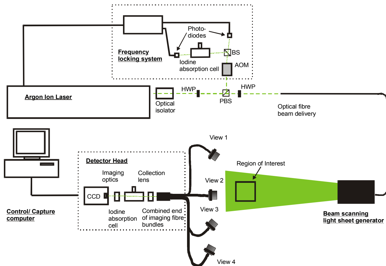
Figure 10. Schematic showing the experimental arrangement used for the three dimensional velocity measurements.
