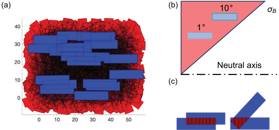
Figure 5. Critical tapes (a) marked in blue in plane, (b) through depth, and (c) their overlapped area with other tapes.
