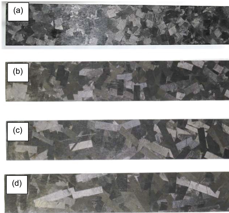
Figure 9. Flexural specimens with different tape lengths of (a) 6 mm, (b) 12 mm, (c) 18 mm, and (d) 24 mm.
