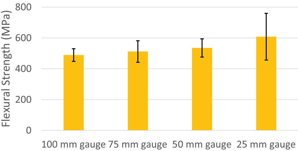
Figure 11. Scaling effect of predicted flexural strength and scatter.
