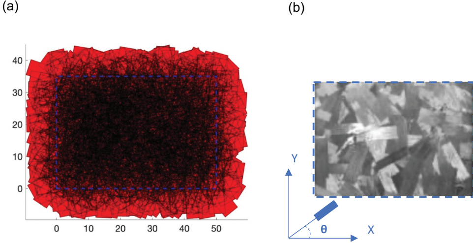
Figure 4. A laminate consists of randomly oriented tapes with (a) a blue boxing indicating the modelled region, (b) angle of the tapes defined with the actual specimen.
