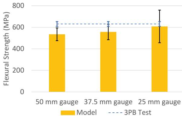
Figure 8. Comparison of modelling results of different model gauge lengths and the 3-point bending experimental results.
