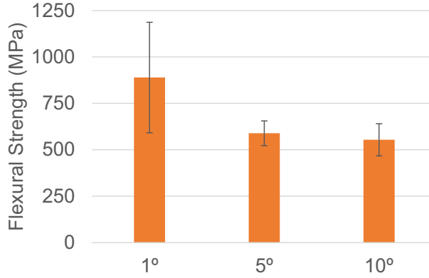
Figure 6. Predicted flexural strength converges with different maximum critical tape angles.
