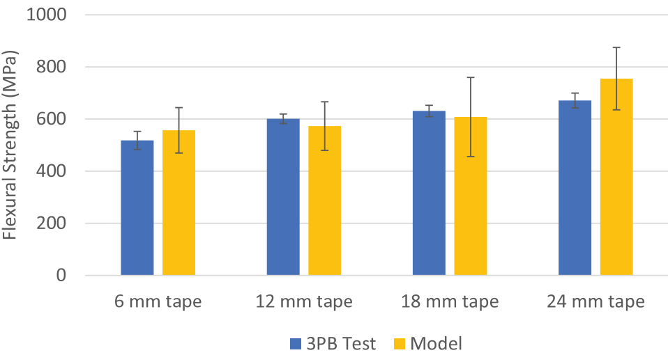
Figure 10. The effect of tape length on flexural strength under 3-point bending.
