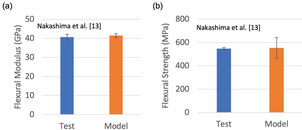
Figure 7. Results comparison between 4-point bending tests and the model for (a) flexural modulus, and (b) flexural strength.
