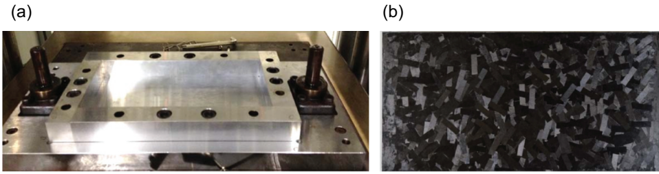
Figure 1. UT-ROS manufacture (a) mould, (b) moulded plate with 18 \times 5 mm tapes.
