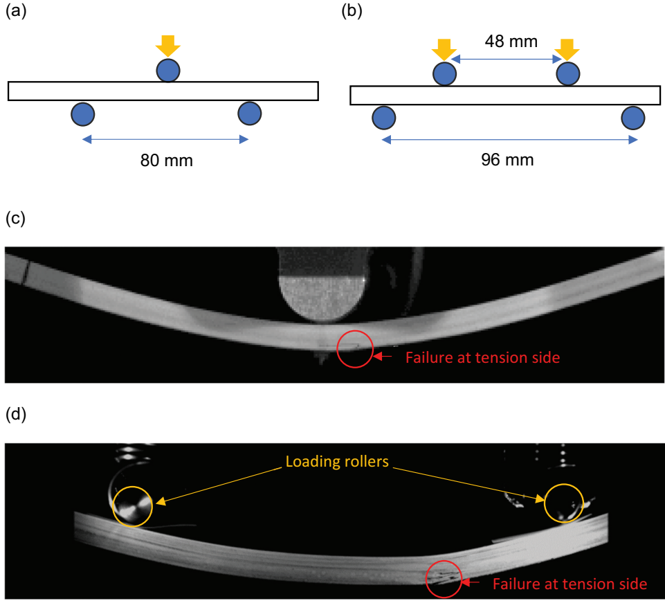
Figure 2. Flexural tests under (a) 3-point bending, (b) 4-point bending, (c) a picture showing fibre-dominant tensile first failure under 3-point bending, and (d) under 4-point bending.
