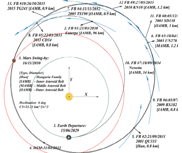
Figure 1. CASTAway asteroid tour trajectory as presented in Sanchez et al. [7].
