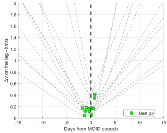
Figure 6. \Delta v variation on the different legs of a asteroid tour (reference trajectory as in Table 2) with respect to the MOID epochs for each of the visited asteroids.
