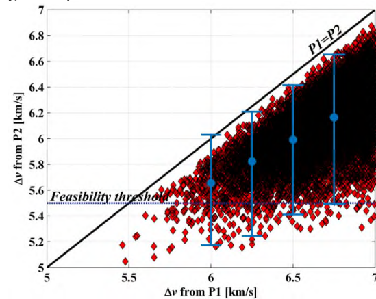
Figure 4. Summary of continuous-variables optimized solutions (P2) and their combinatorial transcription (P1) estimates.
