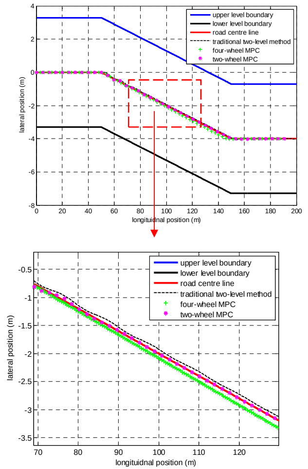
Figure 3. Vehicle desired and actual trajectory in the first set of simulations.
