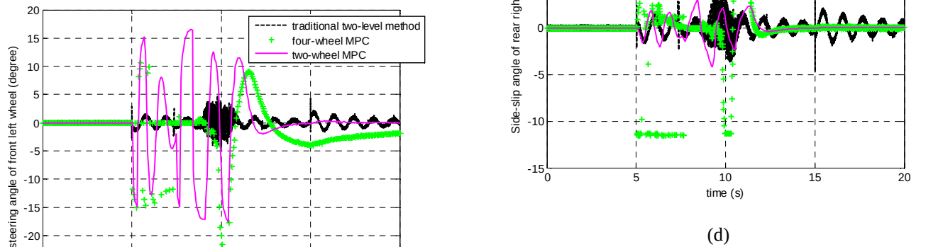
Figure 10. Vehicle steering angle and side-slip angle responses in the third set of simulations.
