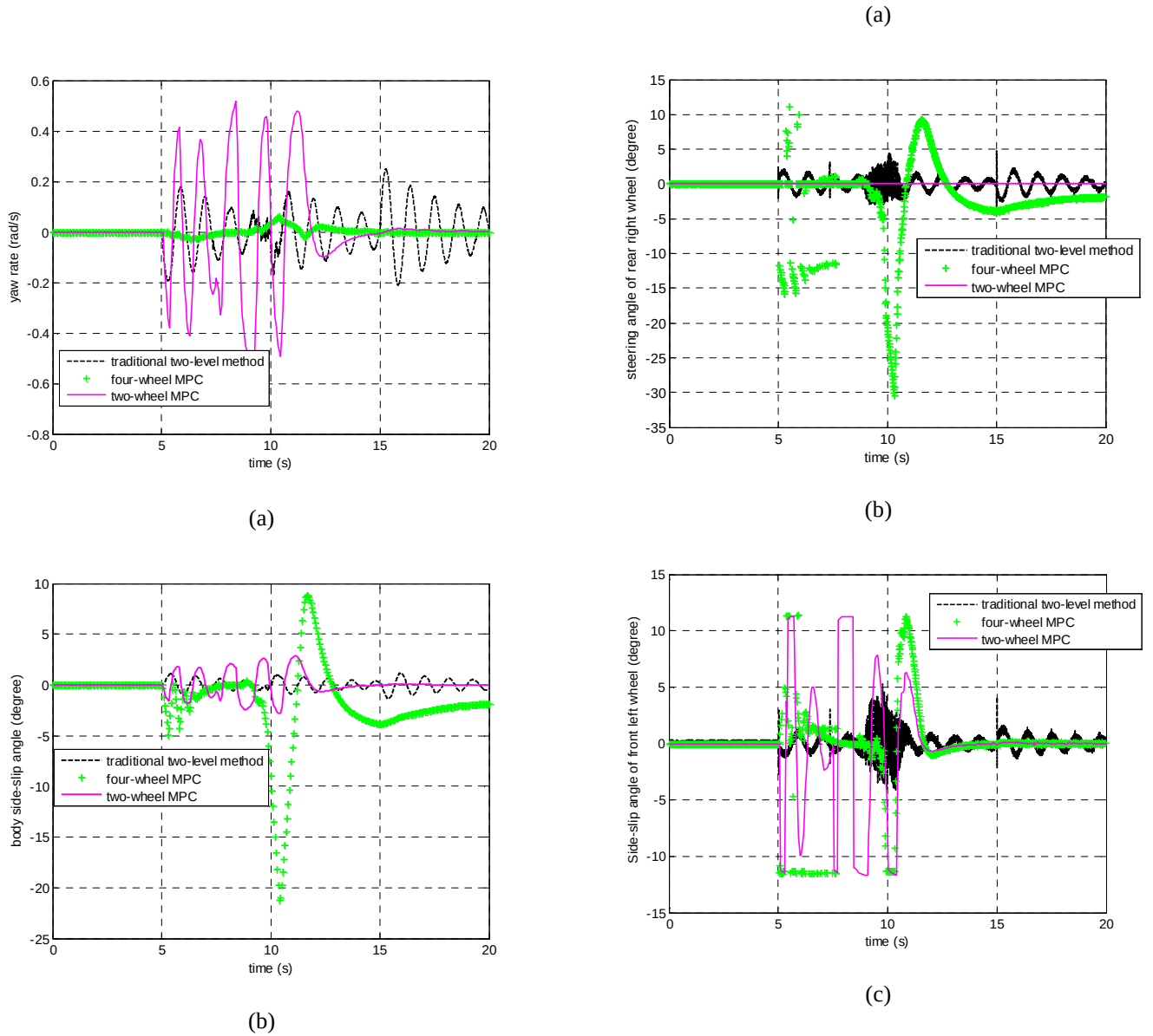
Figure 9. Vehicle dynamics response in the third set of simulations.
