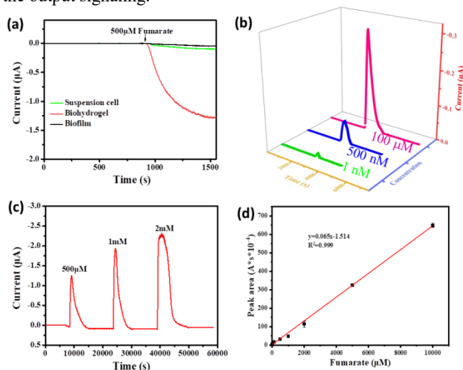
Figure 4. (a-c) Amperometric response of the biosensing system to fumarate. (d) Calibration curve for fumarate quantification with the biohydrogel.
