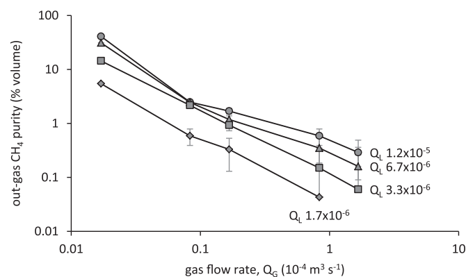
Fig. 6. Impact of Q G ( 1.7 \times 10^{-6} – 1.7 \times 10^{-4} \text{ m}^3 \text{ s}^{-1} ) upon out-gas CH 4 purity for fixed values of Q L .
