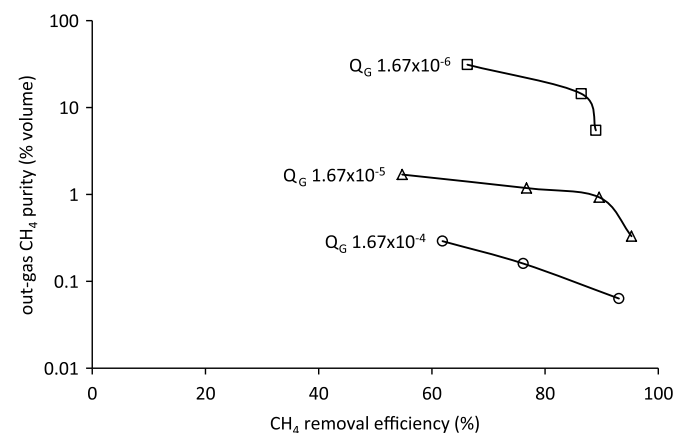
Fig. 8. Trade-off between removal efficiency and purity of recovered CH 4 .
