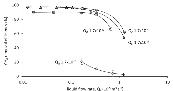
Fig. 2. \text{CH}_4 removal efficiencies from water saturated by a \text{CH}_4/\text{CO}_2 mixture (75/25, 1 atm, 25 ^\circ\text{C} ) for different magnitudes of sweep-gas Q_G ( 1.7 \times 10^{-7} – 1.7 \times 10^{-4} \text{m}^3 \text{s}^{-1} ) against variable Q_L ( 1.3 \times 10^{-7} – 1.3 \times 10^{-5} \text{m}^3 \text{s}^{-1} ) using a HFMC.
