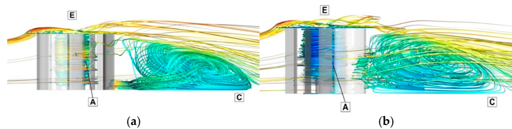
Figure 24. D Streamlines (XZ side view) for a stream velocity of 16.8 m/s for (a) +40; (b) −40 pitch angles.
