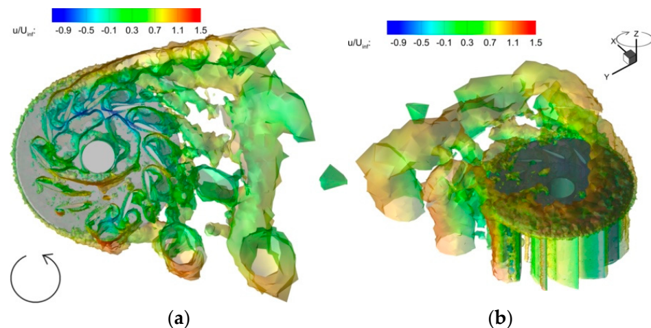
Figure 34. Q-criterion representation for -40° and stream velocity of 16.8 m/s: (a) bottom view; (b) isometric view.
