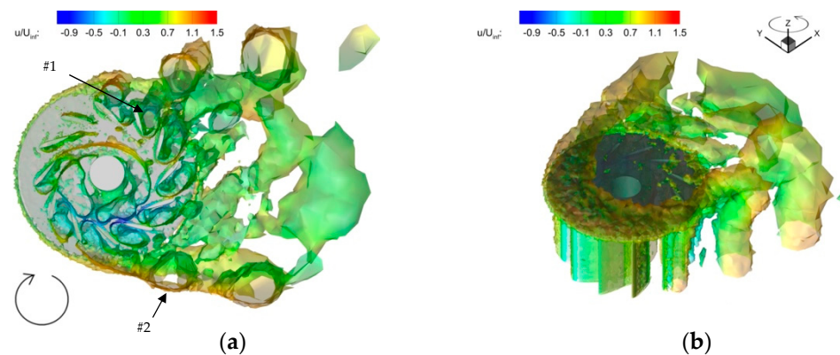
Figure 33. Q-criterion representation for +40° and stream velocity of 16.8 m/s: (a) bottom view; (b) isometric view.
