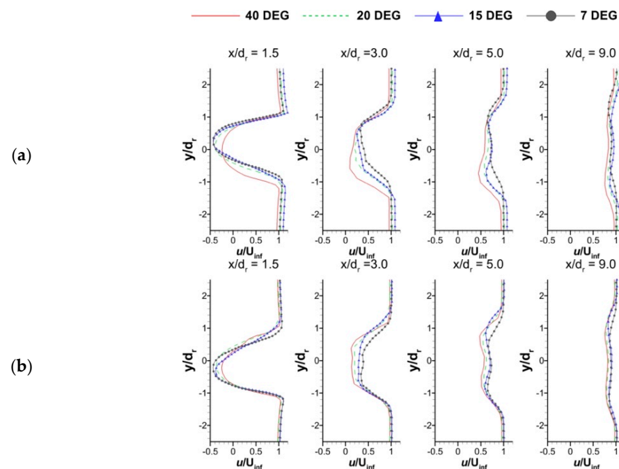
Figure 18. XY mean velocity profiles for stream velocity of 16.8 m/s at different normalised distances for (a) positive pitch angles; (b) negative pitch angles.
