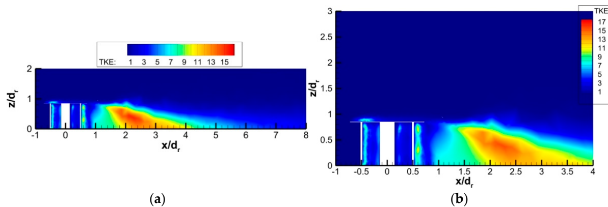
Figure 31. Instantaneous TKE representation in XZ plane for +40^\circ case: (a) wake view; (b) zoom view of turbine.
