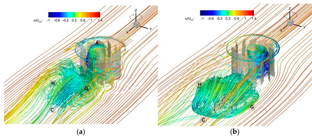
Figure 26. D Streamlines for a stream velocity of 16.8 m/s for (a) +40; (b) −40 pitch angles.
