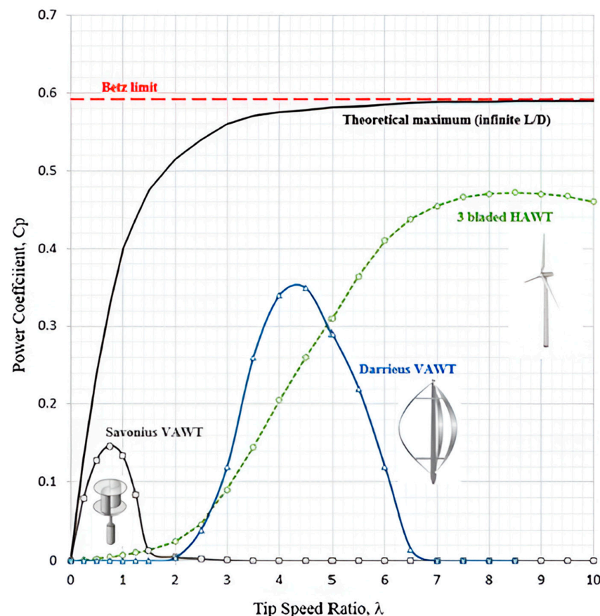
Figure 1. Performance characteristics for three popular designs of wind turbine [9].
