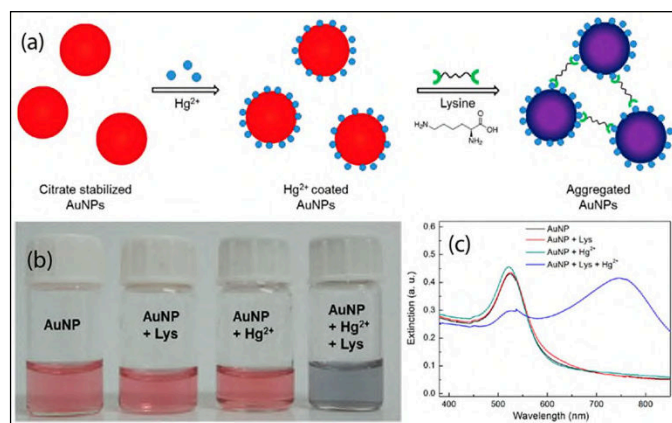
Fig. 12 Schematic representing the \text{Hg}^{2+} sensing mechanism of the colorimetric assay, (b) Photographs of AuNP solutions showing the colour change occurring only in the presence of lysine (0.4 mM) and \text{Hg}^{2+} (10 \mu\text{M} ) and (c) extinction spectra of the AuNP solutions. Reproduced with permission from ref 430
