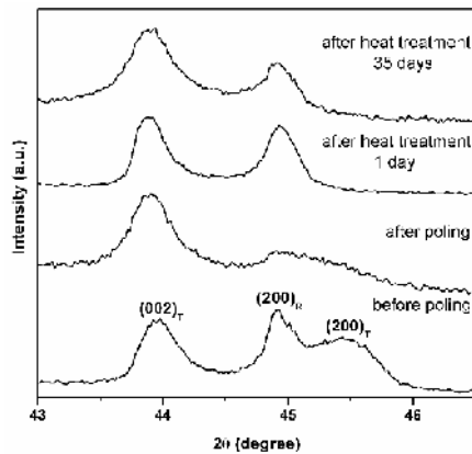
Fig. 2. The XRD patterns at 2\theta ranged from 43-46.5° at difference states of the hard PZT ceramics.
