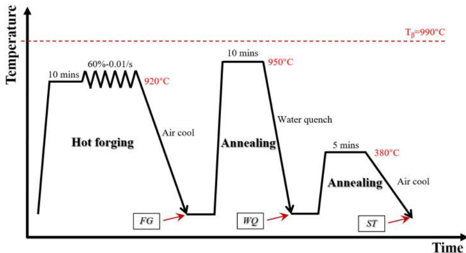
Figure 1. Schematic diagram of three thermal-mechanical processing routes.
