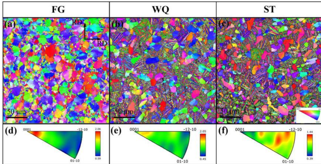
Figure 2. (a–c) EBSD orientation maps of the FG, WQ, and ST alloys, respectively. RD in the figure represents the radial direction, which is perpendicular to the forging direction of the alloy. It is noted that the tensile direction during tensile tests is parallel to the RD. (d–f) IPFs (referenced to RD) of the FG, WQ, and ST alloys, respectively.
