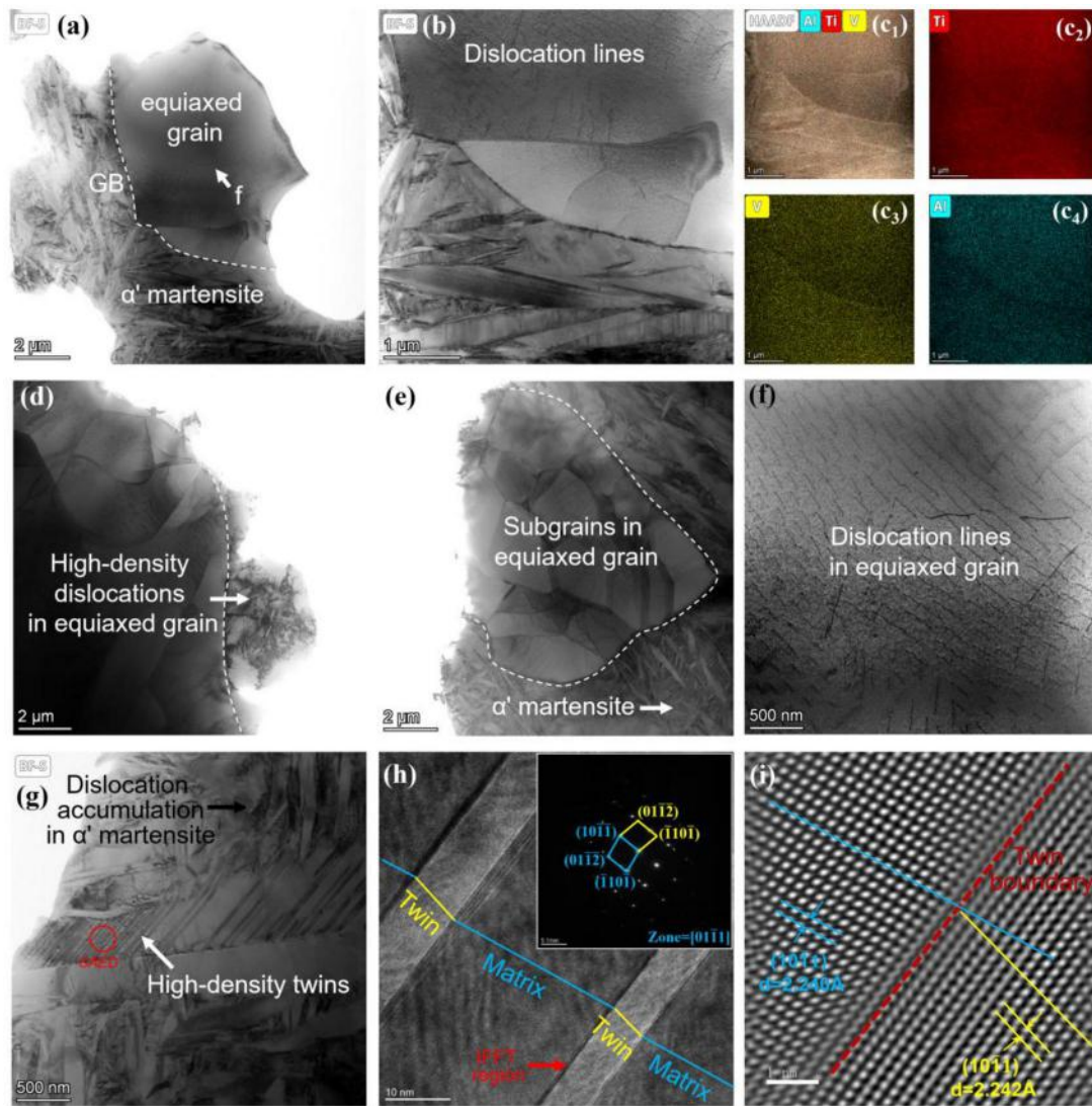
Figure 6. TEM microstructures of the WQ alloy. (a), (b) BF-S images. (c 1 ) High-angle annular dark-field (HAADF) image together with the EDS image for Ti, V, and Al. (c 2 –c 4 ) EDS images showing the elemental distribution of Ti, V, and Al, respectively. (d), (e) BF-S images showing the microstructure of the large equiaxed grains. (f) Magnified image of the marked region in (a). (g) BF-S images showing the twins in acicular \alpha' martensite. (h) HRTEM image of the twinned region in (g), the inset shows the SAED pattern of the marked region in (g). (i) IFFT image of the marked region in (h).
