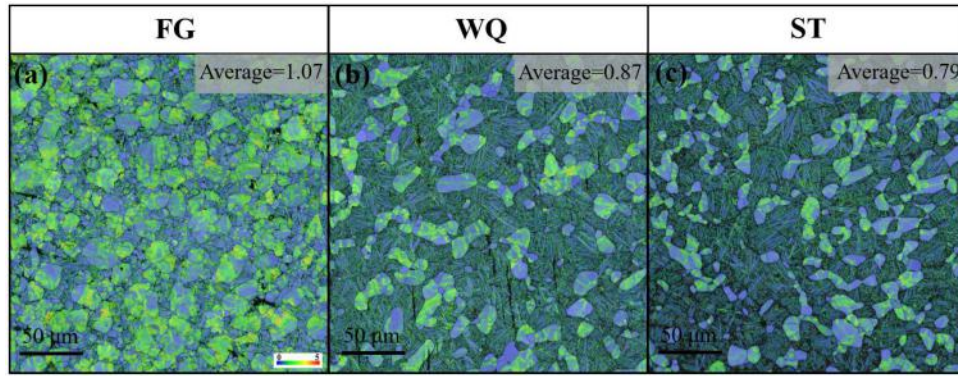
Figure 4. (a–c) KAM maps of the FG, WQ, and ST alloys, respectively. The average KAM values are shown in the figures.
