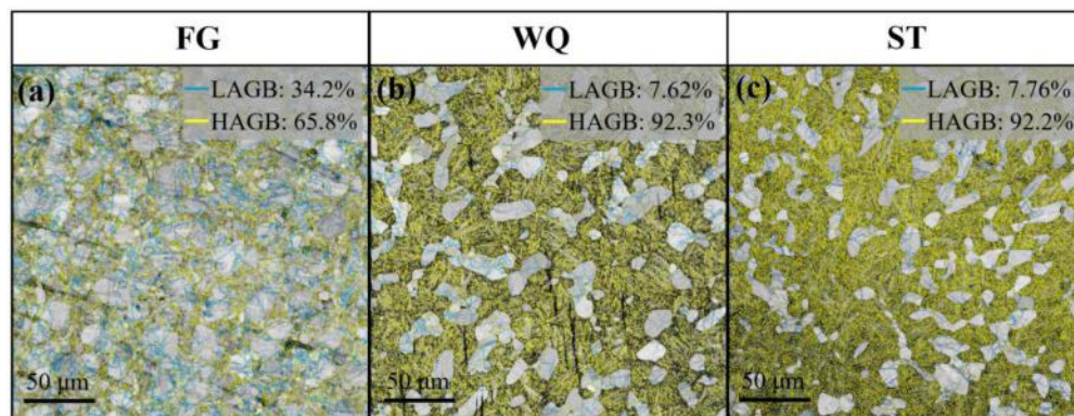
Figure 3. (a–c) Grain boundary maps of the FG, WQ, and ST alloys, respectively. The fraction of HAGB and LAGB are shown in the figures.
