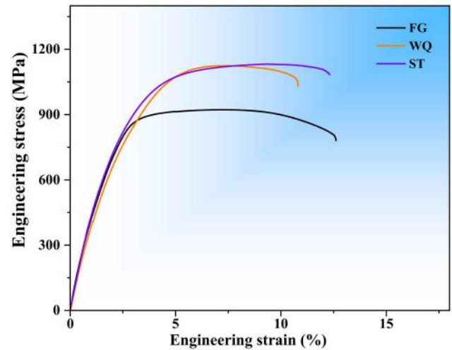
Figure 5. Engineering stress-strain curves of the FG, WQ, and ST alloys.
