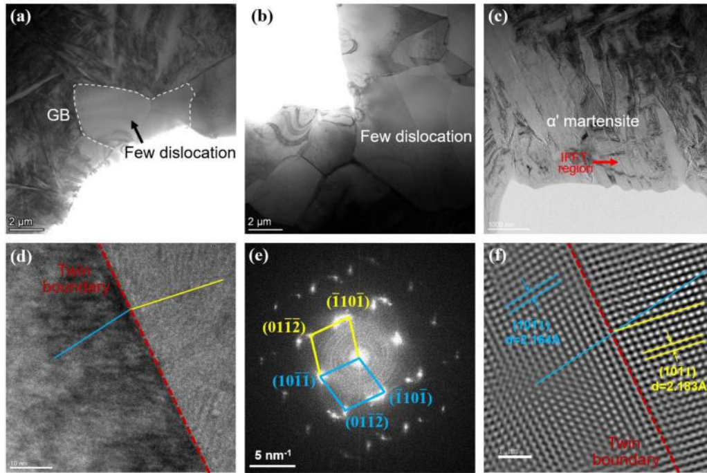
Figure 7. TEM microstructures of the ST alloy. (a–c) BF-S images. (d) HRTEM image of the twinned region in (c). (e) FFT diffraction pattern of the region shown in (d). (f) IFFT image of the twin boundary region shown in (d).
