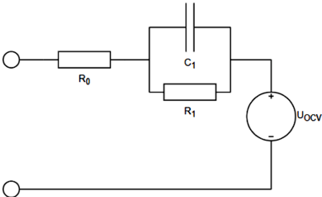
Figure 4. Electrical ECM.
