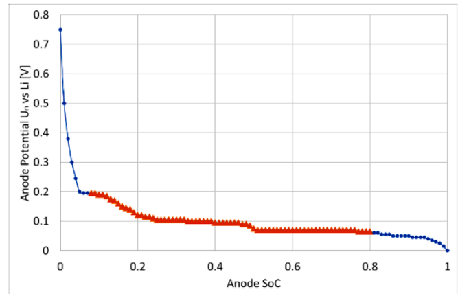
Figure 8. Anode Potential Curve [52].
