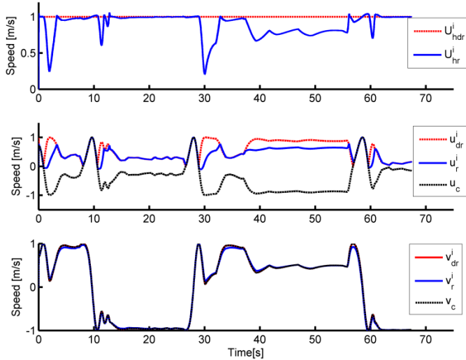
Fig. 5. Velocity and heading tracking during path-following with current disturbance of \beta_c = \pi/4 and V_c = 1\text{ m/s} .
