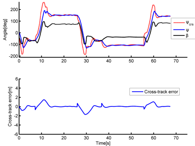
Fig. 6. Heading angles and cross-track error during path-following at \beta_c = \pi/4 and V_c = 1\text{ m/s} .
