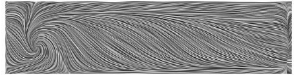
c) Cavity roof ( x - y plane at z/D = 1 )
