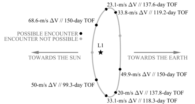
Fig. 7. \Delta V and TOF requirements to reach asteroid 2011 GA along L1 halo orbit (ephemeris model, impulsive trajectories).
