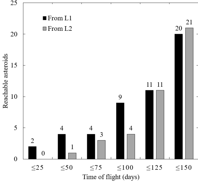
Fig. 4. Cumulative number of reachable asteroids from L1 and L2 as a function of TOF (CR3BP model, impulsive trajectories, \Delta V \leq 80 m/s).
