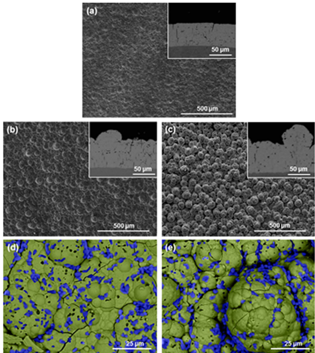
Figure 6. SEM images from the surface of samples produced with a bath load of 100 g/l, a current densities of 37 A/dm 2 and different brushes: (a) grey Scotch-Brite™, (b) polyester, and (c) white Scotch-Brite™. The main image is taken with secondary electrons and the inserts are BS images of cross-sections, enabling visualization of aluminium particles (black dots). (d) and (e) are a higher magnification, back-scattered images of (b) and (c) respectively, false-coloured to show Al particles in blue and the Ni matrix in green.
