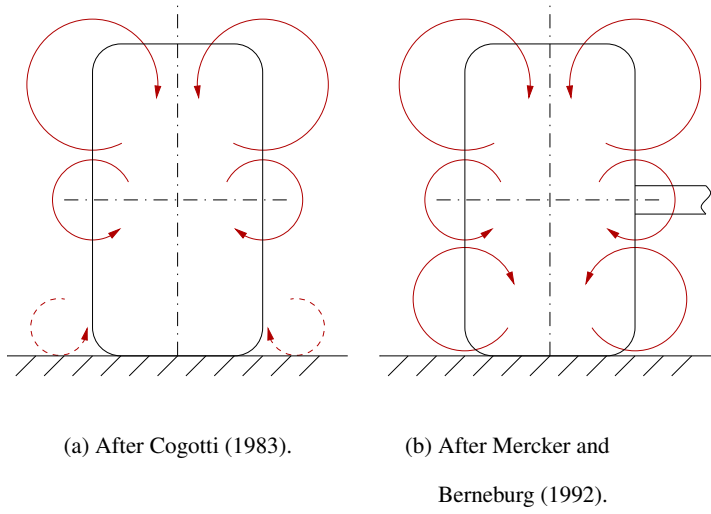
Figure 2 Models of the trailing vortex system induced by a wheel rotating on the ground.
