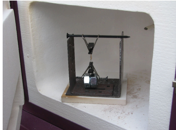
Fig. 10. Thermomechanical Demise Test Set-Up
