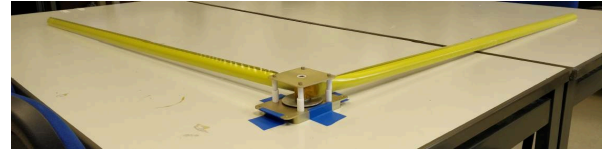
Fig. 7. Test Set-Up: Two Perpendicular Lenticular Sheathed Booms, Supported Deployment
