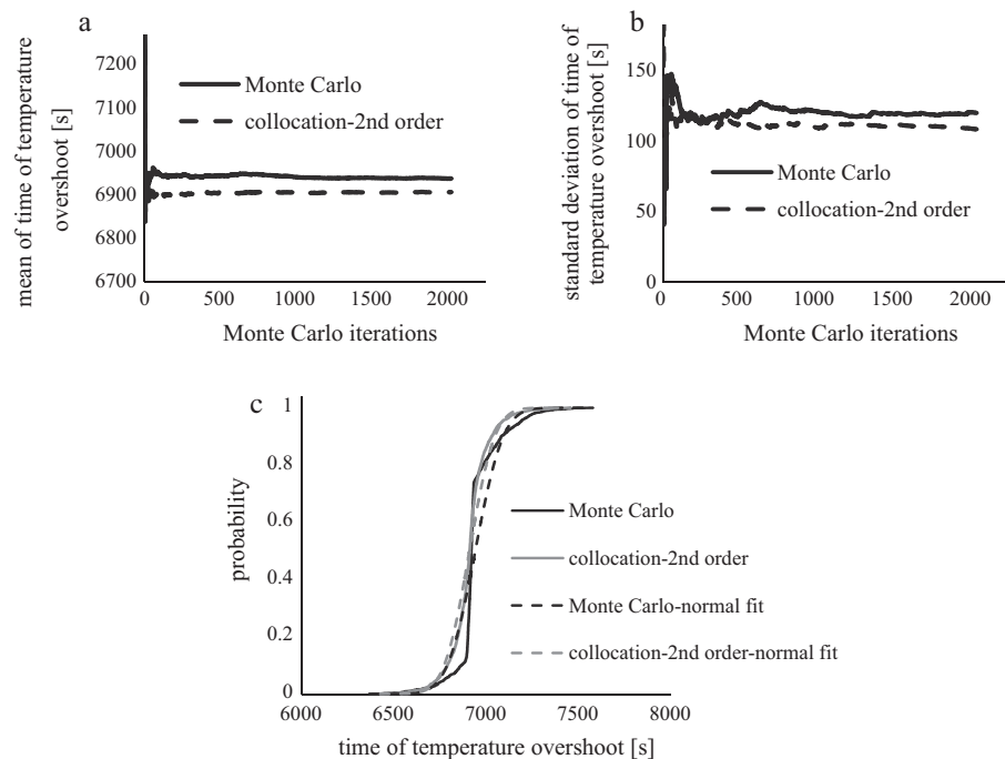
Fig. 5. Convergence of statistics of mean (a) and standard deviation (b) of time temperature overshoot (c) probability distribution of time of temperature overshoot.
