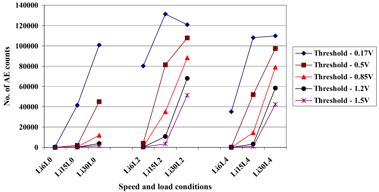
Figures 22 Number of AE counts for a ‘large’ inner race defect at varying speeds and load conditions
