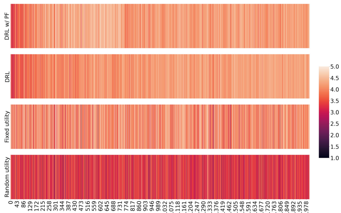
Fig. 6 Average satisfaction level of each episode of NYC scenario
