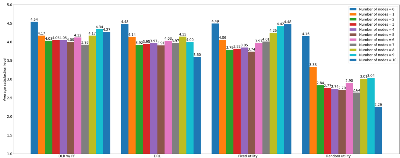
Fig. 8 Average satisfaction level by number of nodes of NYC scenario
