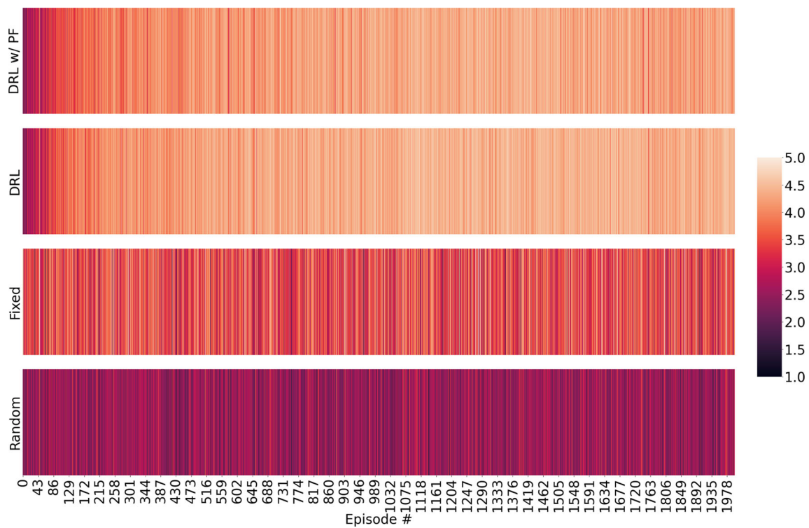
Fig. 10 Average satisfaction level of each episode of synthetic scenario
