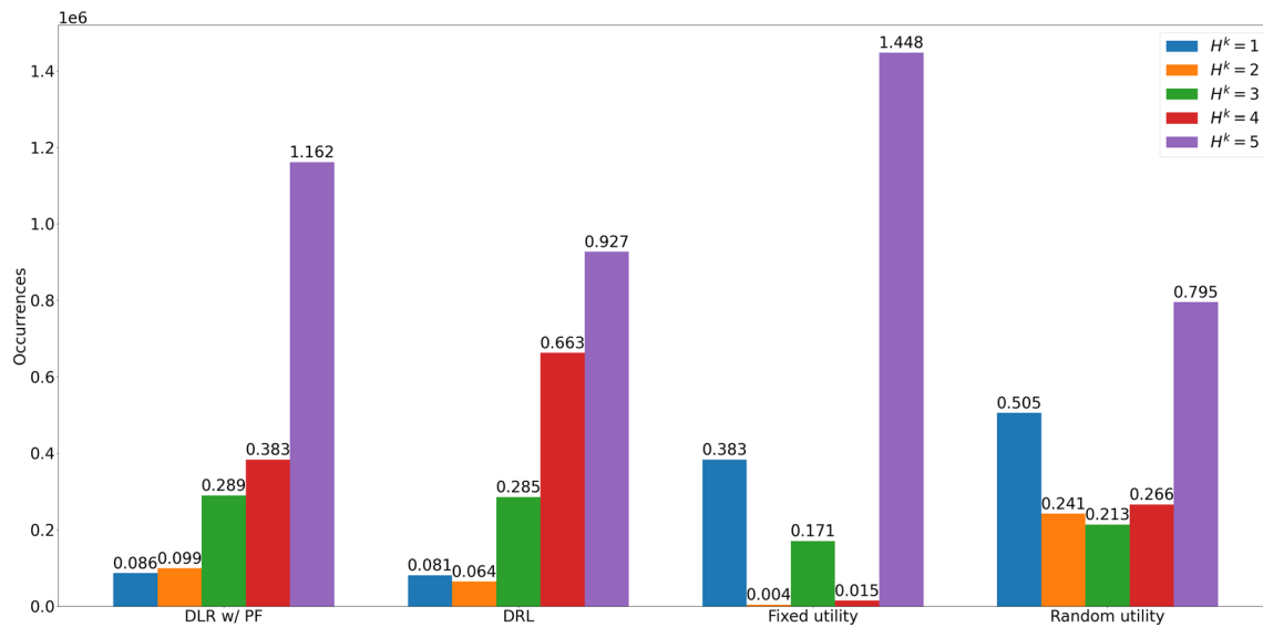
Fig. 7 Total number of satisfaction level of each method of NYC scenario
