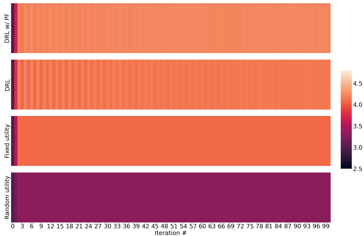
Fig. 5 Average satisfaction level of each iteration of NYC scenario
