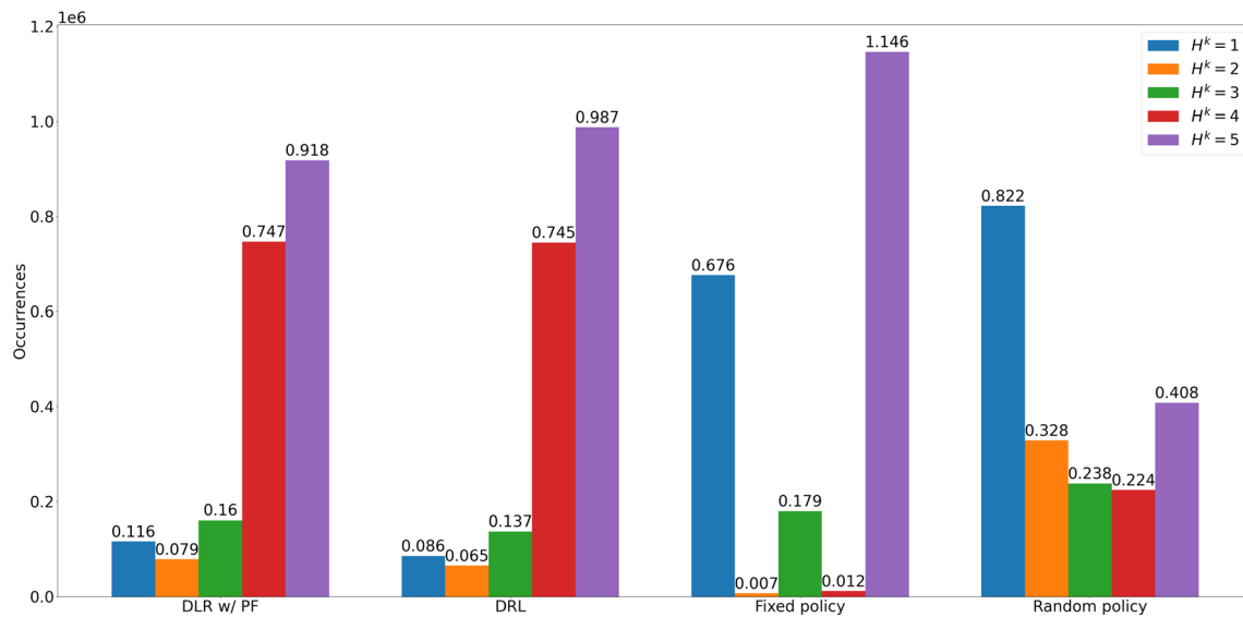
Fig. 11 Total number of satisfaction level of each method of synthetic scenario
