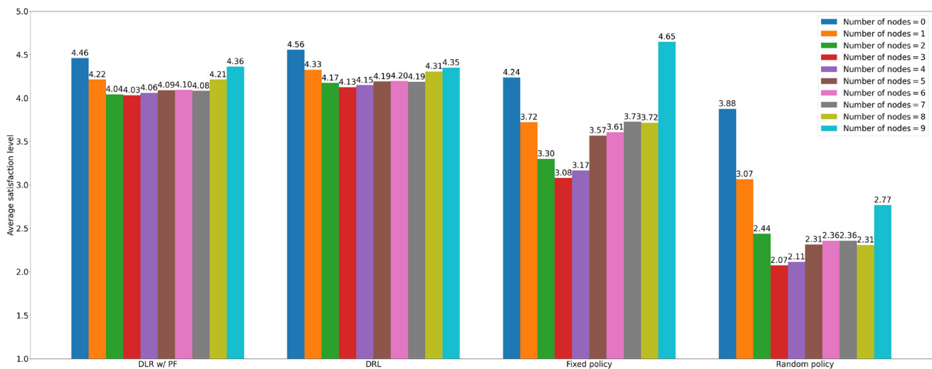
Fig. 12 Average satisfaction level by number of nodes of synthetic scenario
