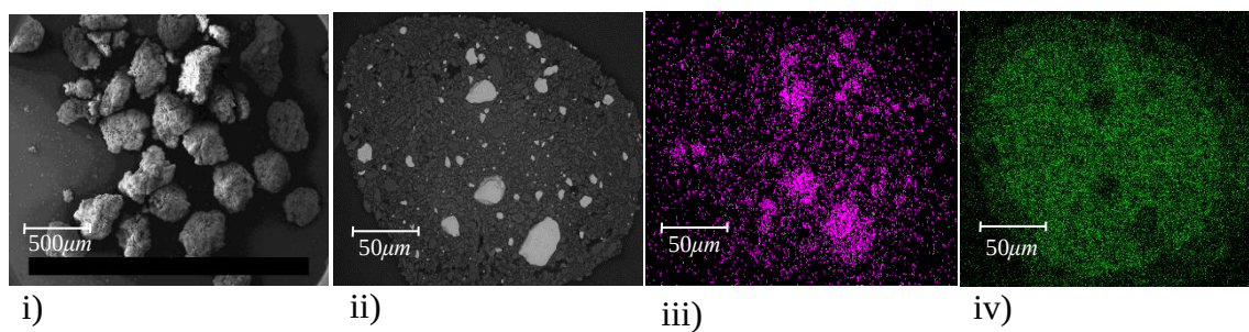
Figure 5: Cu25Al75 i) High-resolution SFEG image (scale 500 \mu\text{m} ), ii) Global particle view EDX, iii) Cu elemental mapping EDX, iv) Al elemental mapping EDX
