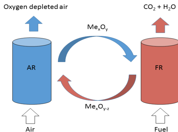
Figure 1: Simplified CLC process, adapted from [5]
