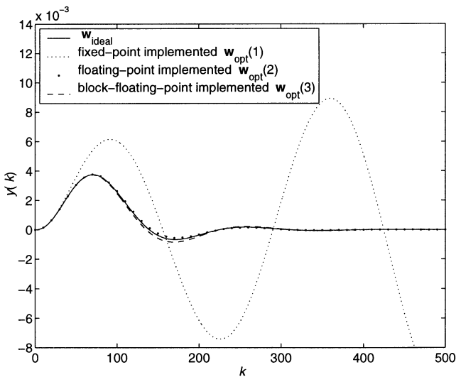
Fig. 4. Unit impulse response of y(k) for w_{\text{ideal}} , 18-bit fixed-point implemented w_{\text{opt}}(1) (eight integer bits and nine fractional bits), 18-bit floating-point implemented w_{\text{opt}}(2) (four exponent bits and 13 mantissa bits), and 18-bit block-floating-point implemented w_{\text{opt}}(3) (three block exponent bits and 14 block mantissa bits) of Example 2.
