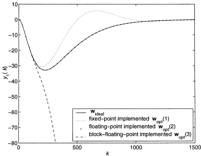
Fig. 3. Unit impulse response of y_1(k) for w_{\text{ideal}} , 22-bit fixed-point implemented w_{\text{opt}}(1) (three integer bits and 18 fractional bits), 22-bit floating-point implemented w_{\text{opt}}(2) (five exponent bits and 16 mantissa bits), and 22-bit block-floating-point implemented w_{\text{opt}}(3) (two block exponent bits and 19 block mantissa bits) of Example 1.
