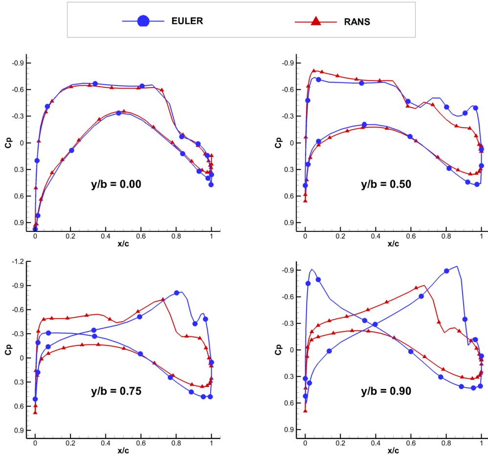
Fig. 6. Comparison between low fidelity (EULER) and high fidelity (RANS) solution in terms of pressure distribution.
