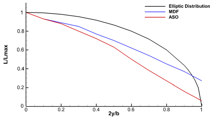
Fig. 15. Comparison between the normalized lift distribution resulting from the MDF and ASO formulations and that of the aerodynamic optimum.
