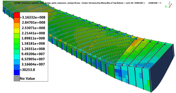
(b) Minimum Drag design, max Von Mises stress: 319 MPa
