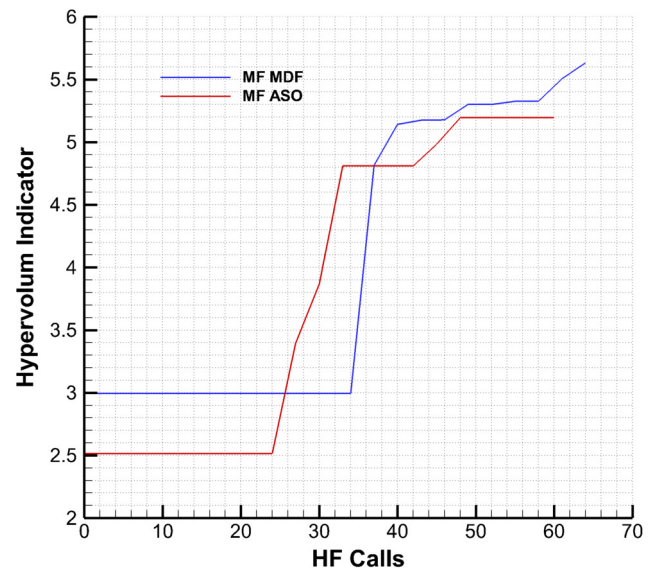
Fig. 14. Comparison between the convergence of pareto front generated using the MDF and the ASO formulation using the hypervolume indicator.
