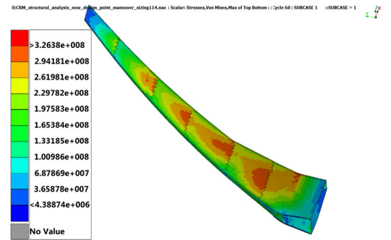
(f) Minimum Drag design, max Von Mises stress: 319 MPa
