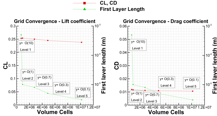
Fig. 4. Global aerodynamic coefficients grid convergence study for the HF analysis.
