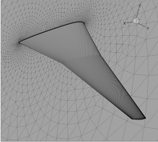
Fig. 5. High fidelity aerodynamic surface grid. O-type grid layers are used for boundary layer resolution.
