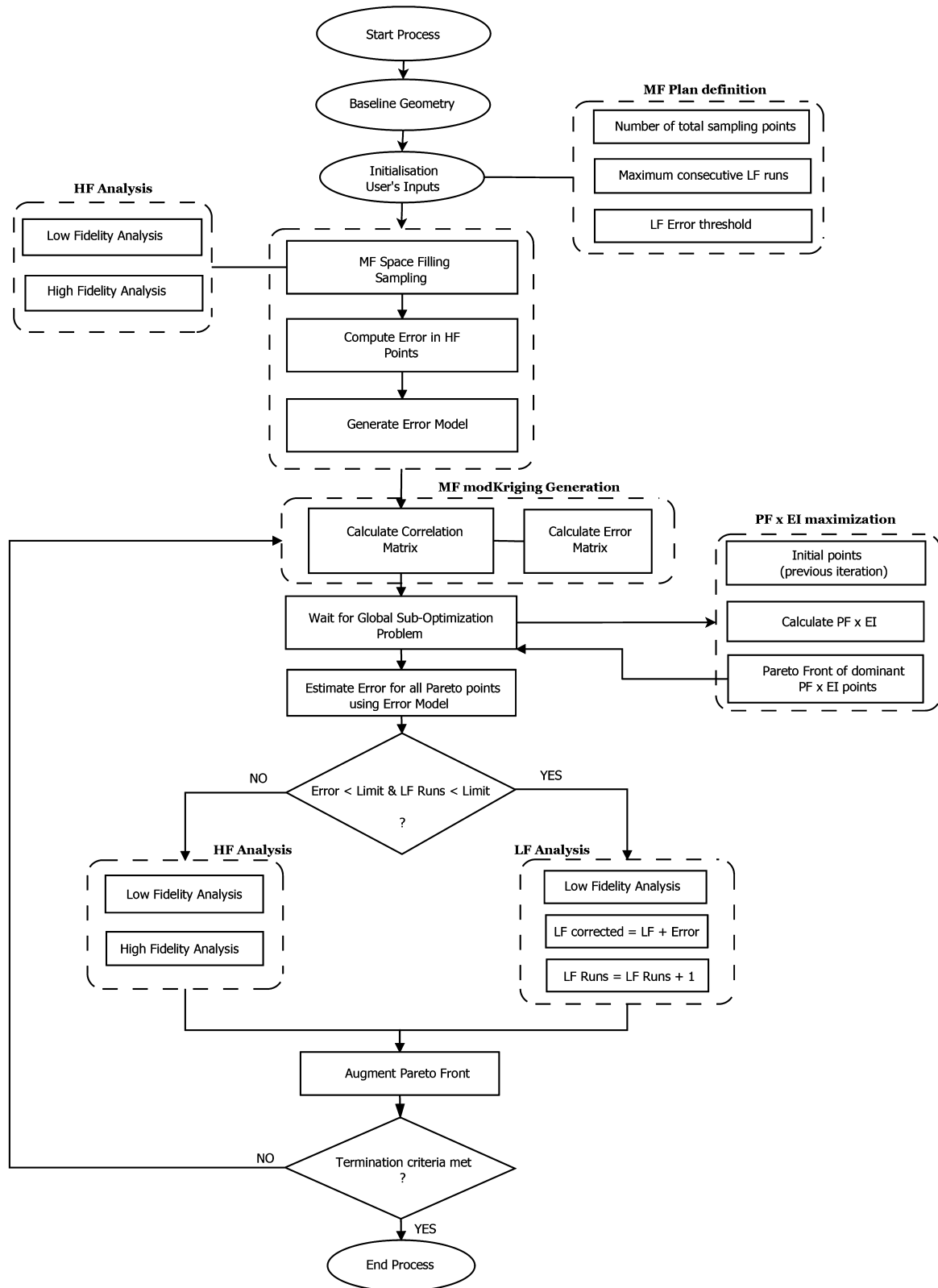
Fig. 1. Methodology used for the optimization of the CRM.
