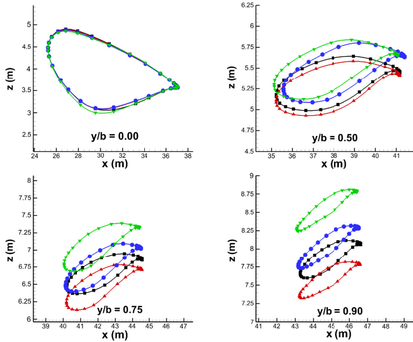
(b) Wing sections in different locations across the span.
