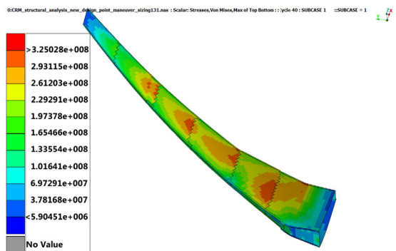
(g) Compromise design, max Von Mises stress: 319 MPa
