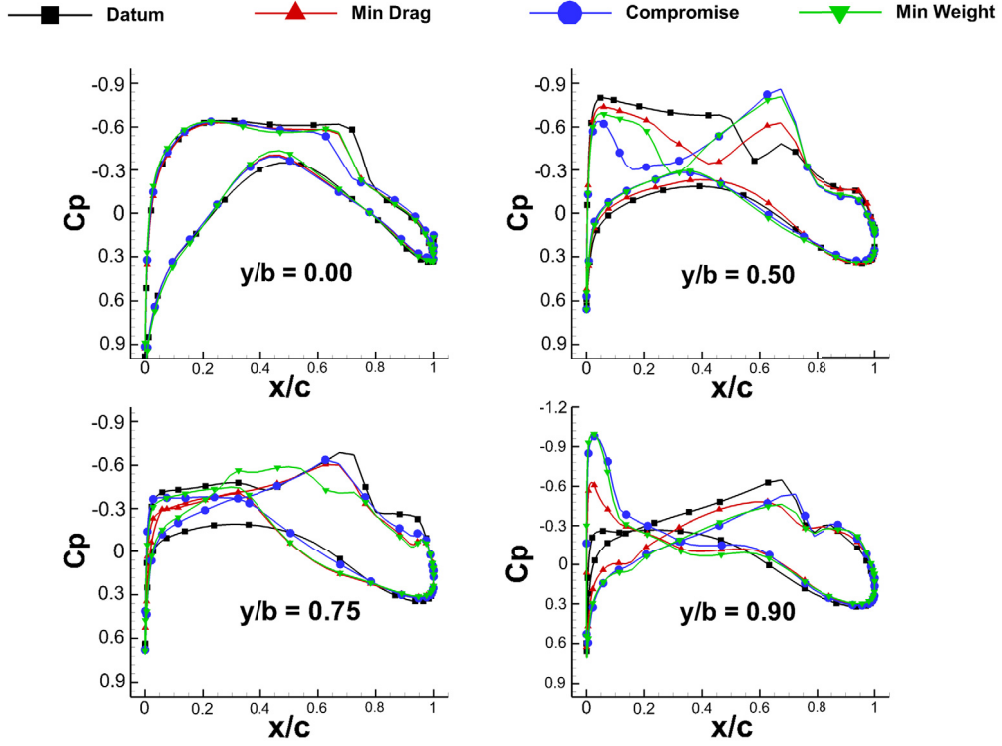
(a) Pressure distribution in different locations across the span.
