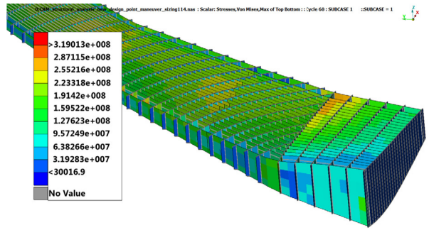
(b) Minimum Drag design, max Von Mises stress: 319 MPa
