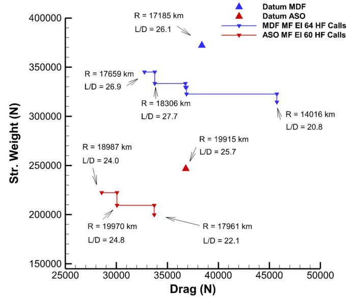
Fig. 13. Comparison between the pareto front generated using the MDF and the ASO formulation.
