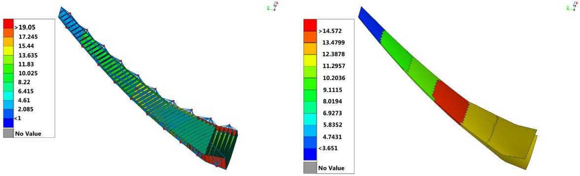
(a) CONM2 masses represent fuel and high lift systems' masses, connected with the structure with RBE3 elements. For clarity, shear webs are omitted.
