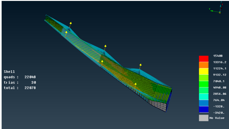
Fig. 8. Aerodynamic loads mapping: Pressure loads are interpolated with RBF functions, while LE/TE forces are transferred to the beams using RBE3 elements.
