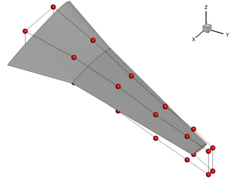
Fig. 2. FFD control points deforming the OML and the wingbox.
