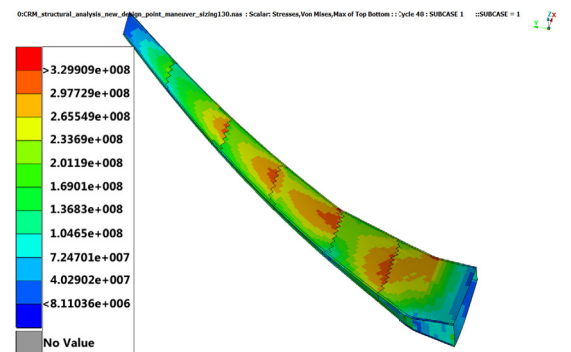
(h) Minimum Weight design, max Von Mises stress: 316 MPa
