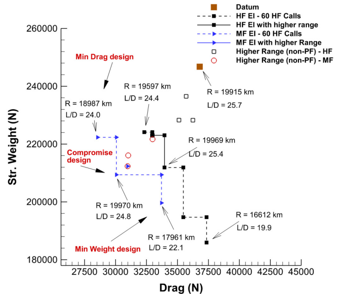
Fig. 9. Pareto front comparison between the HF and the MF methods, using Feasibility to handle the constraints for the ASO formulation. As in MDF, a tradeoff is required between aerodynamics and structures to achieve range performance.
