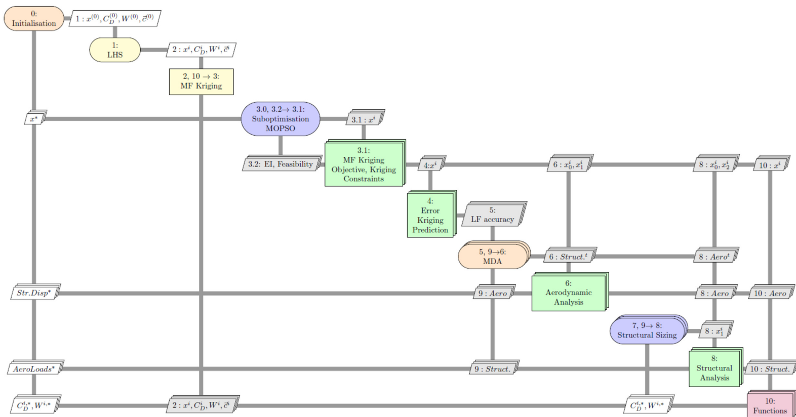
Fig. 7. XDSM flowchart for ASO formulation of CRM aerostructural optimization.
