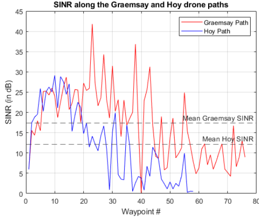
Fig. 7. SINR variation along Graemsay and Hoy UAS paths.
