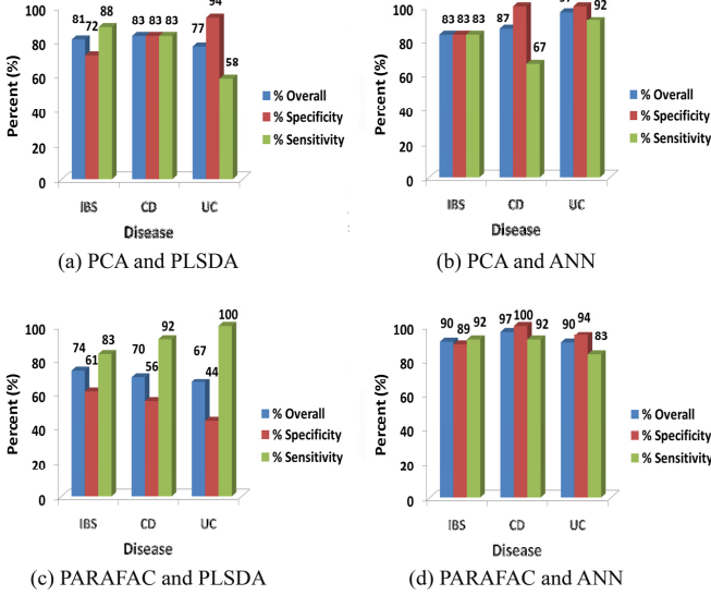
Fig. 4. Comparison of the PLSDA (a and c) against the ANN probability network (b and d) to discriminate the three diseases from the healthy controls in terms of % Overall*, % Specificity** and % Sensitivity*** after application of PCA (a and b) and PARAFAC (c and d) to each EEM.
