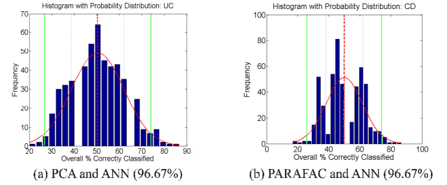
Fig. 5. Monte Carlo simulations applied to the urine samples in which very good overall classifications were attained for PCA (a) and PARAFAC (b).
