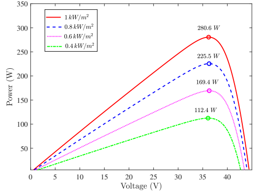
Fig. 9 P-V Characteristic curve of the BP3280T solar panel under various irradiance conditions.
