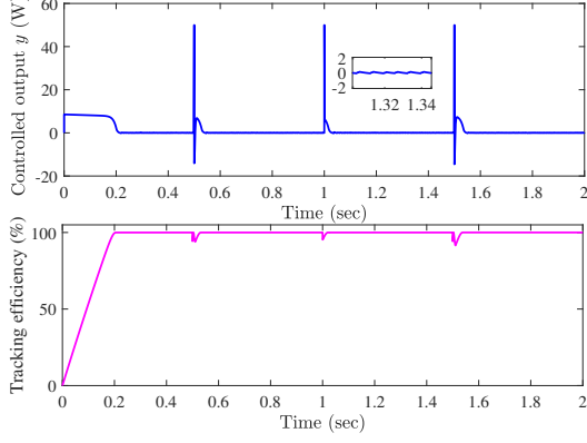
Fig. 15 Analysis performed under varying temperature conditions : Top. Controlled output y . Bottom. Tracking efficiency.
