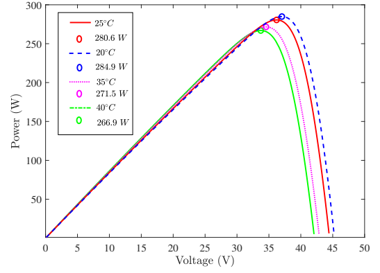
Fig. 14 P-V output curve of the BP3280T solar panel under different temperature conditions.
