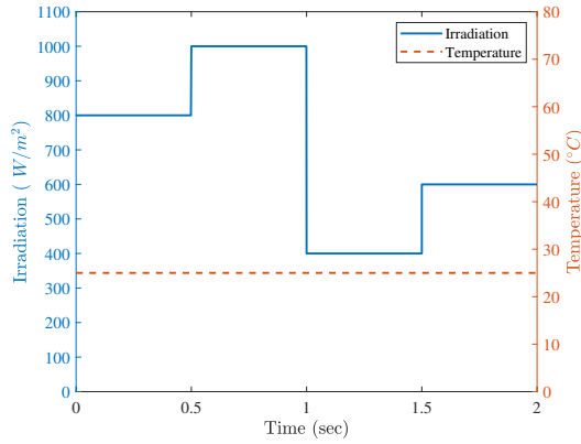
Fig. 8 Overview of variations in solar irradiation conditions at constant temperature.
