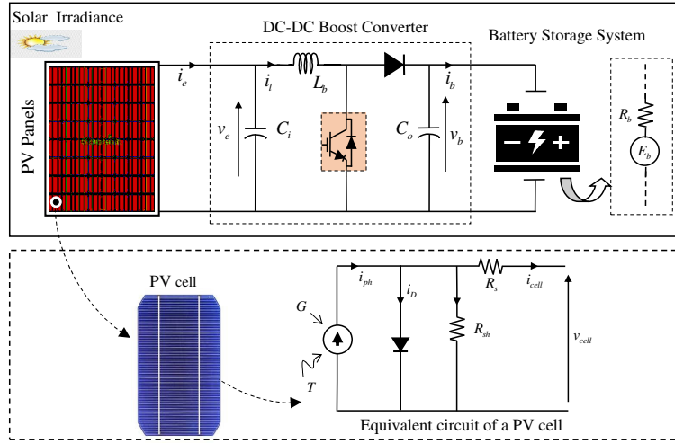
Fig. 1 Schematic diagram of the investigated PV-ES system.
