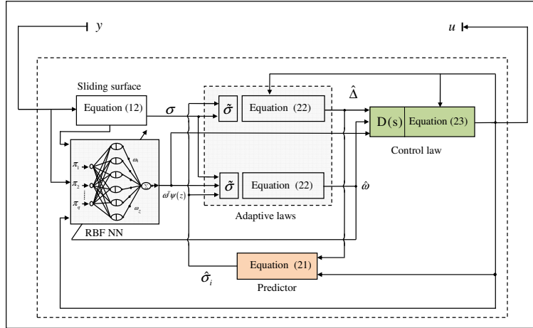
Fig. 2 Block diagram of the suggested \mathcal{L}_1 ANN-MPPT controller.
