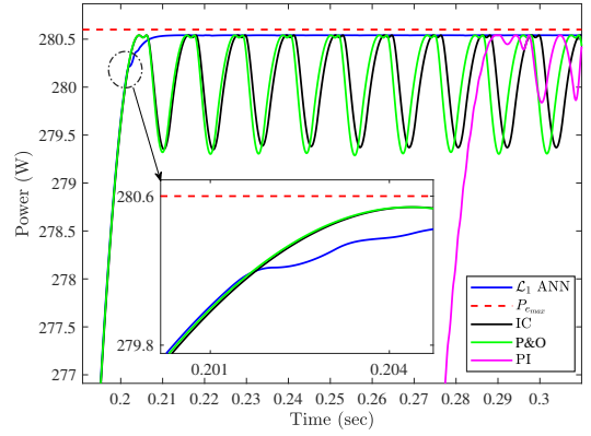
Fig. 18 Dynamic response of the \mathcal{L}_1 ANN-MPPT controller compared with conventional MPPT methods.
