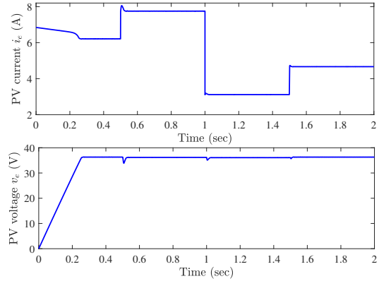
Fig. 11 Analysis performed under varying solar irradiation conditions : Top. PV current i_e . Bottom. PV voltage v_e .
