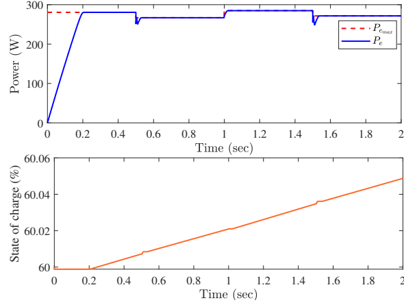
Fig. 12 Analysis performed under varying temperature conditions: Top. PV output power P_e and maximum power P_{e_{max}} . Bottom. Time evolution of SOC.
