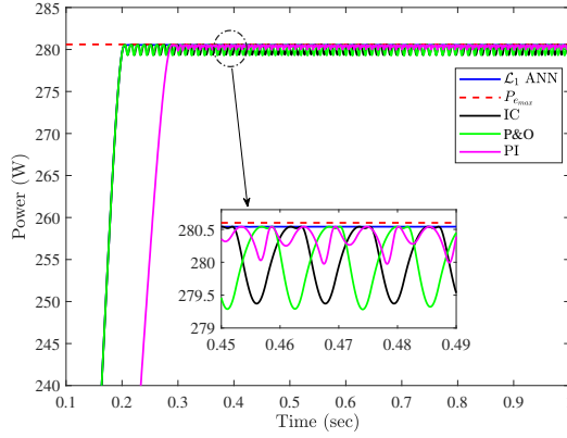
Fig. 17 Tracking performance of the \mathcal{L}_1 ANN-MPPT controller compared with conventional MPPT methods.
