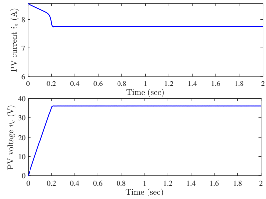
Fig. 6 Analysis performed under normal weather conditions : Top. PV current i_e . Bottom. PV voltage v_e .
