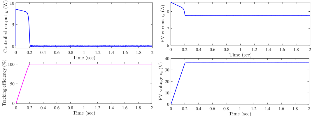
Fig. 5 Analysis performed under normal weather conditions: Top. Controlled output y . Bottom. Tracking efficiency .
