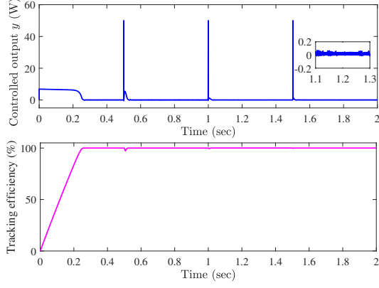
Fig. 10 Analysis performed under varying solar irradiation conditions : Top. Controlled output y . Bottom. Tracking efficiency.
