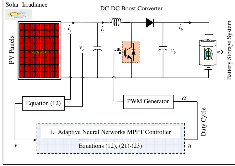
Fig. 3 \mathcal{L}_1 ANN-MPPT controller designed for a PV-ES system.
