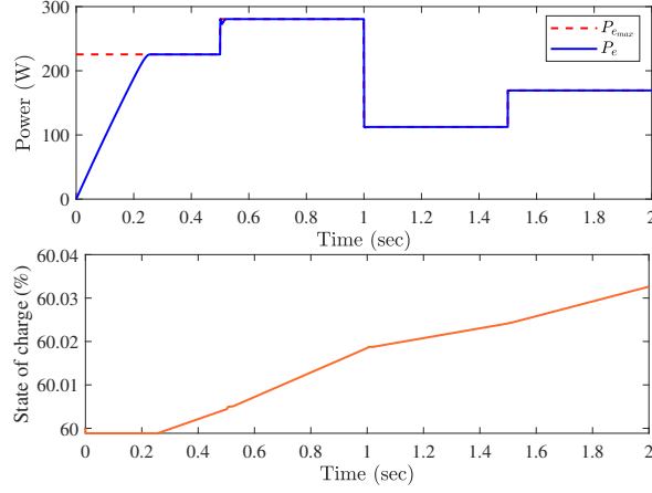
Fig. 7 Analysis performed under varying solar irradiation conditions: Top. PV output power P_e and maximum power P_{e,max} . Bottom. Time evolution of SOC.
