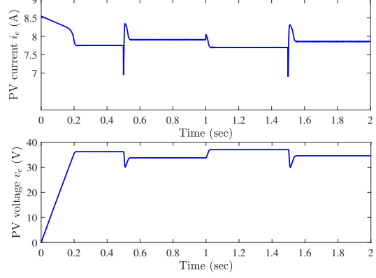
Fig. 16 Analysis performed under varying temperature conditions : Top. PV current i_e . Bottom. PV voltage v_e .
