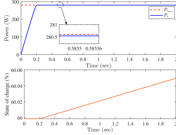
Fig. 4 Analysis performed under normal weather conditions: Top. PV output power P_e and maximum power P_{e_{max}} . Bottom. Time evolution of SOC.
