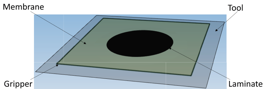
Fig. 1. Mirror geometry: (a) spherical dish (RoC = 8 m); (b) aperture view (D = 0.50 m, central aperture = 50 mm); (c) forming simulation setup showing rigid tool, membrane, and laminate configuration used for forming analysis.
