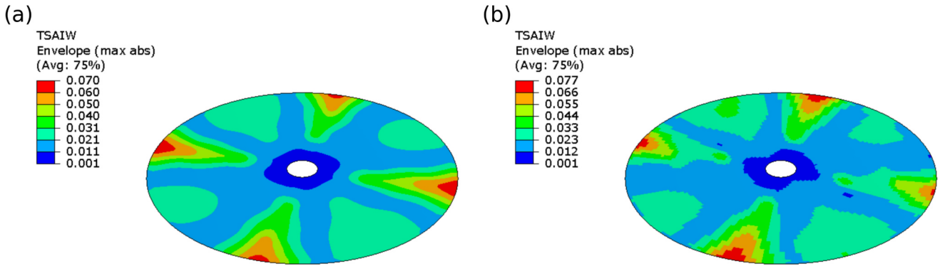
Fig. 9. Random vibration (static-equivalent axial) strength assessment: (a) straight-fibre at 152.72 Hz with equivalent \sim 93 g (max Tsai-Wu \approx 0.07 ); (b) RTS at 145.02 Hz with equivalent \sim 90.55 g (max Tsai-Wu \approx 0.08 ).
