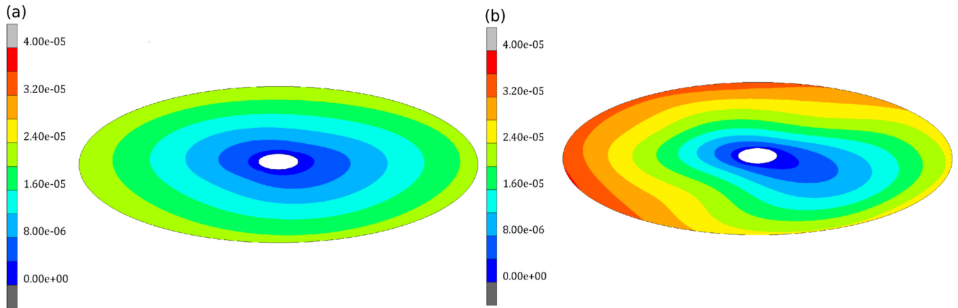
Fig. 11. Moisture-desorption deformation fields (m): (a) straight-fibre; (b) RTS.
