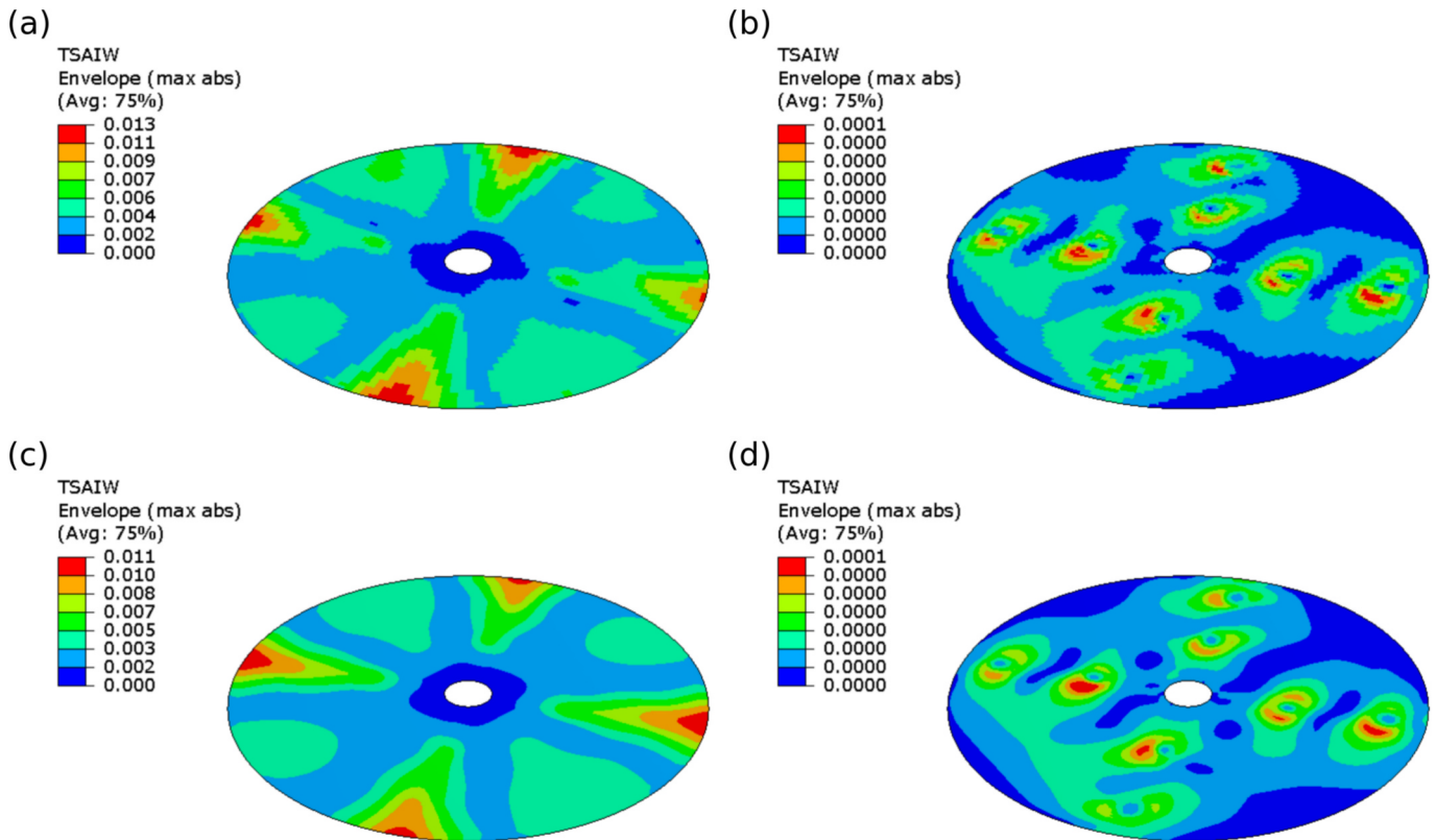
Fig. 8. Tsai-Wu failure index under launch quasi-static accelerations: (a) straight-fibre, 15 g axial; (b) straight-fibre, 4 g lateral; (c) RTS, 15 g axial; (d) RTS, 4 g lateral.
