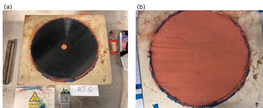
Fig. 6. Thermomechanical test setup: (a) mirror on hot plate; (b) copper powder interface for improved thermal contact and minimal constraint.
