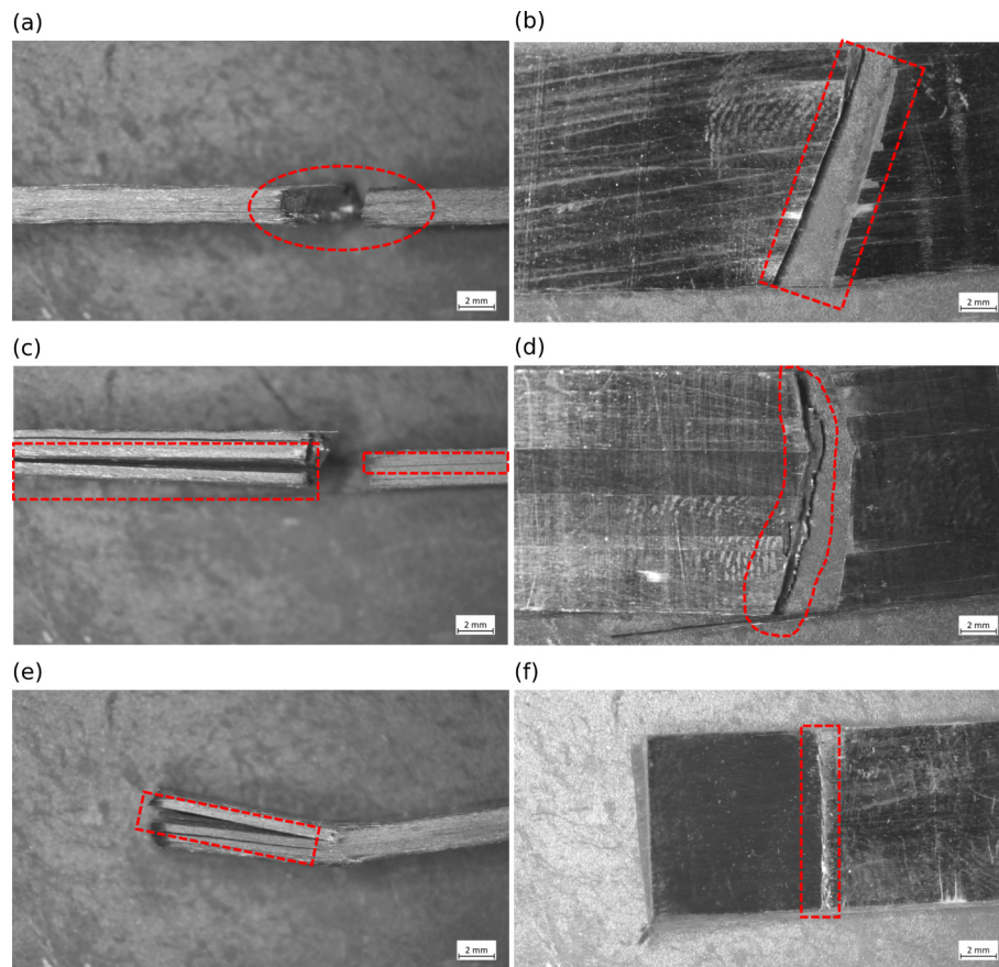
Fig. 15. Microscopy of failure modes in reference coupons: (a, b) three-point bending; (c, d) four-point bending; (e, f) interlaminar shear (short-beam).
