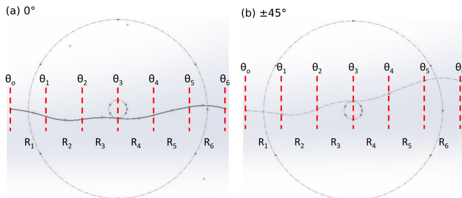
Fig. 3. Spatial distribution of steering angles and radii for RTS plies: (a) 0^\circ plies, (b) \pm 45^\circ plies.
