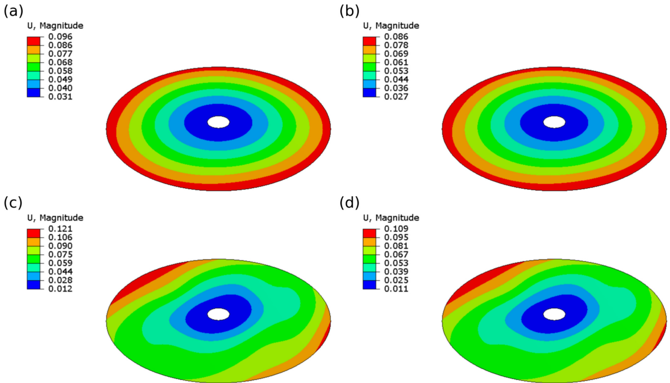
Fig. 10. Out-of-plane displacement (mm) under uniform temperature change: straight-fibre (a) hot, (b) cold; RTS (c) hot, (d) cold.
