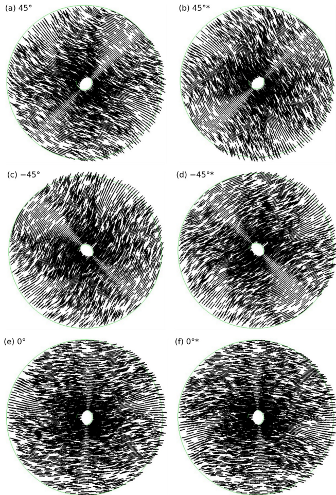
Fig. 2. Orientation distributions for RTS plies showing fibre paths (1-axis direction): (a) 45^\circ , (b) 45^\circ , (c) -45^\circ , (d) -45^\circ , (e) 0^\circ , (f) 0^\circ .
