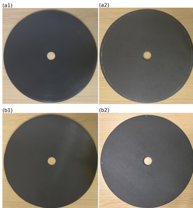
Fig. 5. Manufactured composite reflectors: straight-fibre laminate (a1) optical side, (a2) non-optical side; RTS laminate (b1) optical side, (b2) non-optical side.
