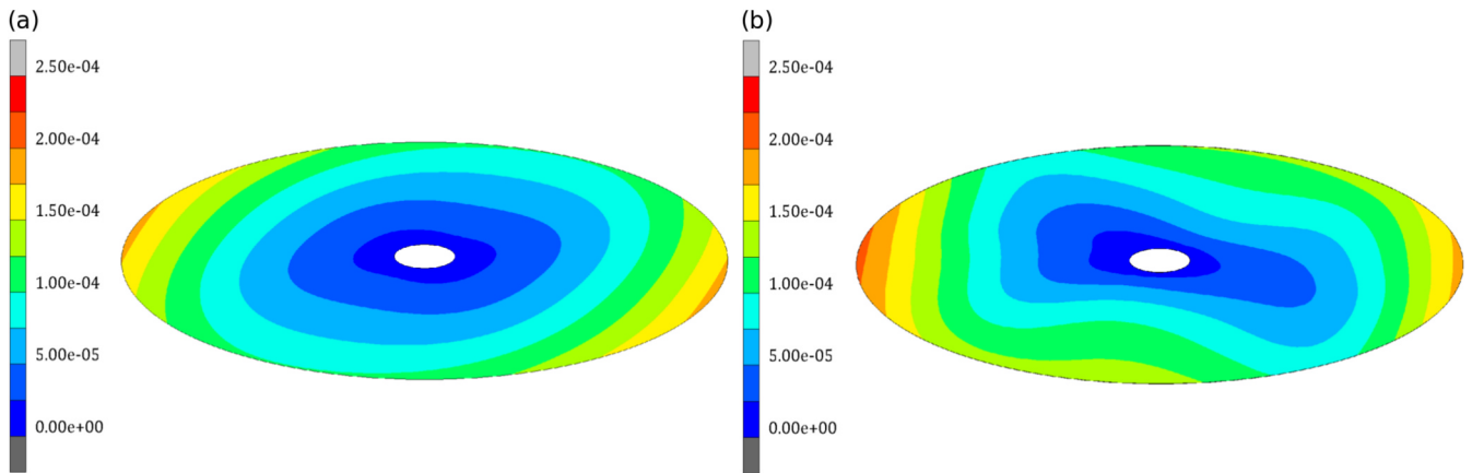
Fig. 12. Predicted post-demoulding distortion from CHILE simulations (m): (a) straight-fibre; (b) RTS.
