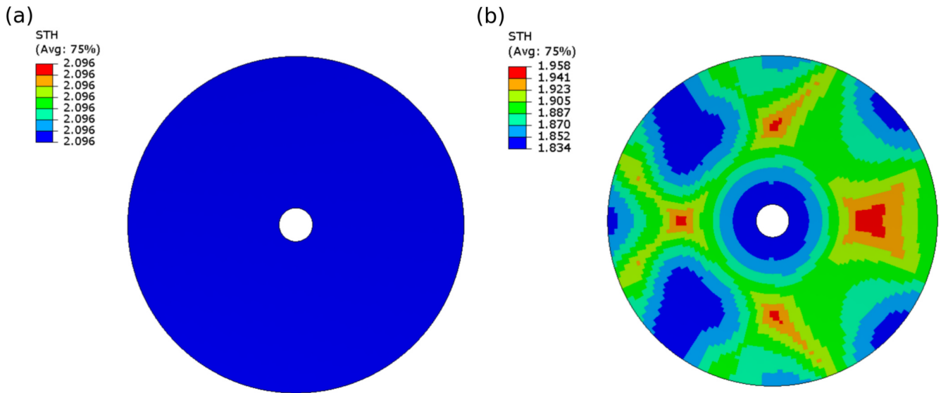
Fig. 7. Laminate thickness: (a) straight-fibre (uniform 2.096 mm); (b) RTS (1.834–1.958 mm due to tow shearing), shown as a colourmap in mm.
