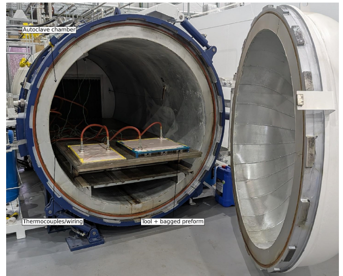
Fig. 4. Autoclave curing of vacuum-bagged preform.
