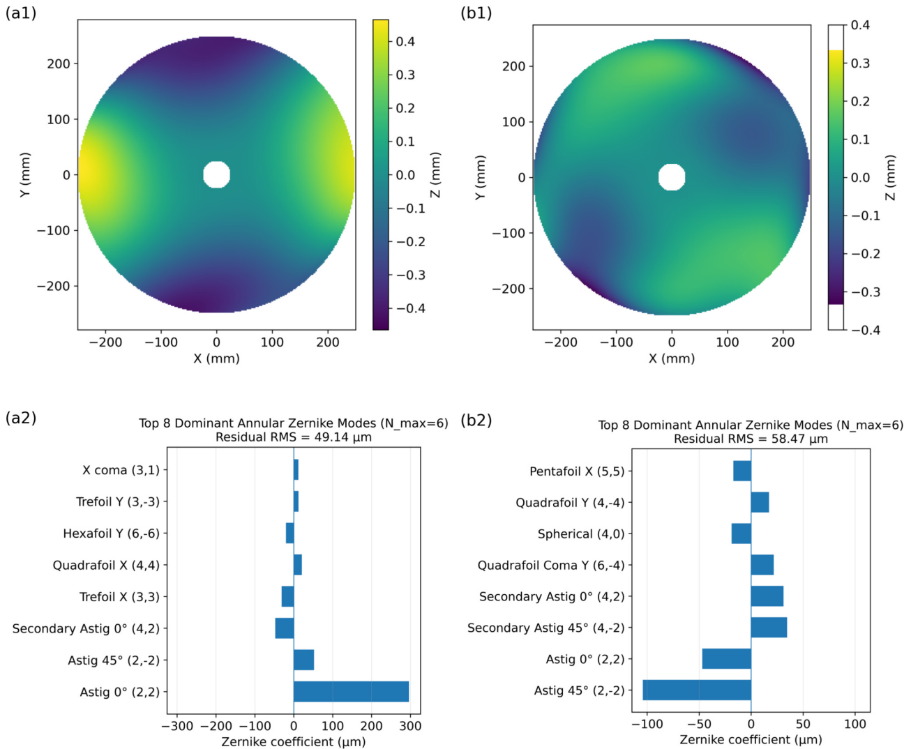
Fig. 13. Residual surface after removing piston, tilt, and defocus: (a1) straight-fibre, (b1) RTS; dominant annular Zernike terms: (a2) straight-fibre, (b2) RTS.
