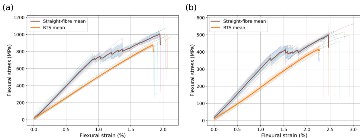
Fig. 14. Flexural stress–strain response: (a) three-point bending; (b) four-point bending (thin lines: specimens; thick line: mean).
