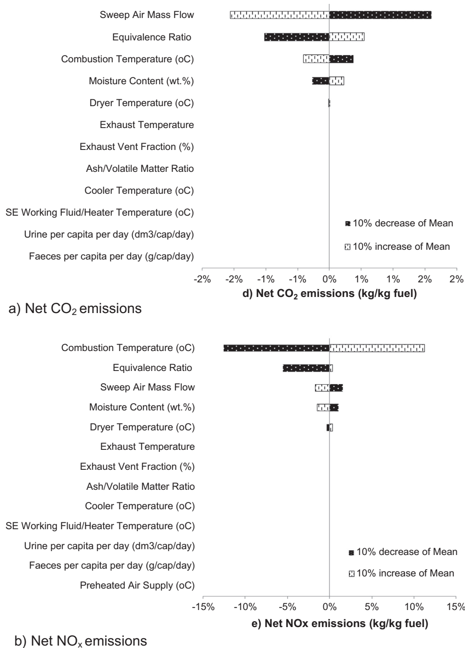
Fig. 9. Percentage contributions of the input variables to emissions.
