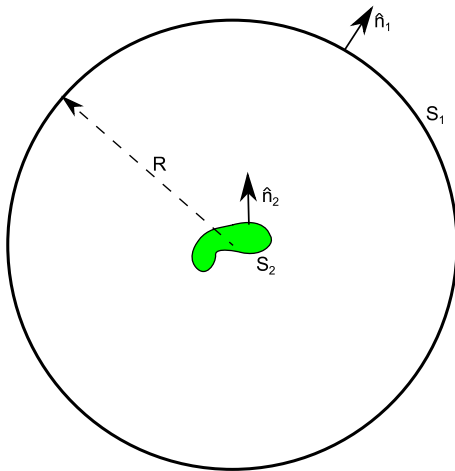
Fig. 6. Region in which the solution is valid is between the two surfaces S_1 , a distant spherical boundary of radius R , and the boundary S_2 , which surrounds the scattering object. \hat{n}_1 and \hat{n}_2 are surface normals on boundary surfaces S_1 and S_2 , respectively.
