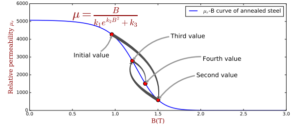
Fig. 5. Relative permeability curve vs flux density of steel.
