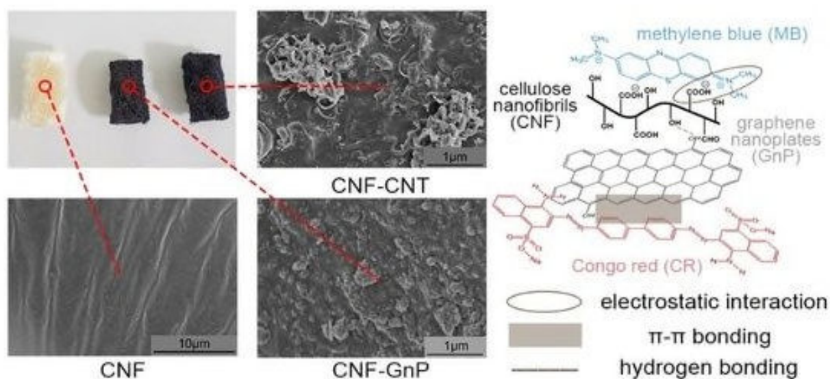
Figure 4. SEM images of hybrid aerogels and a possible mechanisms for the adsorption of congo red and methylene blue dyes [123].
