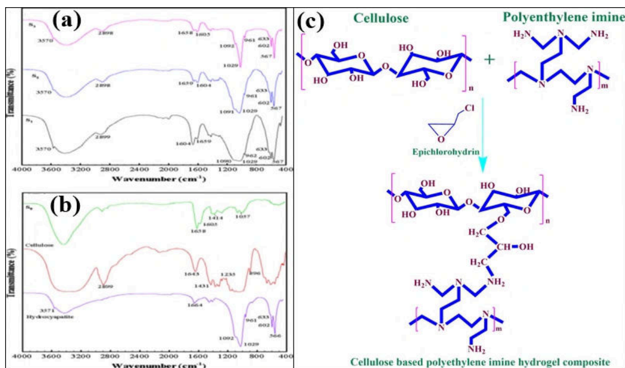
Figure 9. FTIR spectrum of (a) S 1 (hydroxyapatite, Na 2 HPO 4 (0.09 mol L -1 ) and CaCl 2 (0.15mol L -1 )), S 2 (hydroxyapatite, Na 2 HPO 4 (0.18 mol L -1 ) and CaCl 2 (0.31mol L -1 )), S 3 (hydroxyapatite, Na 2 HPO 4 (0.54 mol L -1 ) and CaCl 2 (0.92 mol L -1 )) and (b) S 0 (without hydroxyapatite), pure cellulose and hydroxyapatite [142]. Reprinted with permission from [142]. Copyright 2013 Elsevier, (c) possible mechanism for fabrication of cellulose supported polyethylene imine hydrogel composite [140]. Reprinted with permission from [140]. Copyright 2016 Springer.
