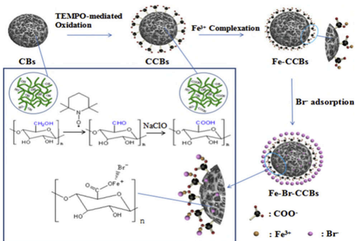
Figure 13. Representation of preparation process and adsorption of \text{Br}^- by using Fe(III)-complexed carboxylated cellulose beads [134]. Reprinted with permission from [134]. Copyright 2020 Elsevier.
