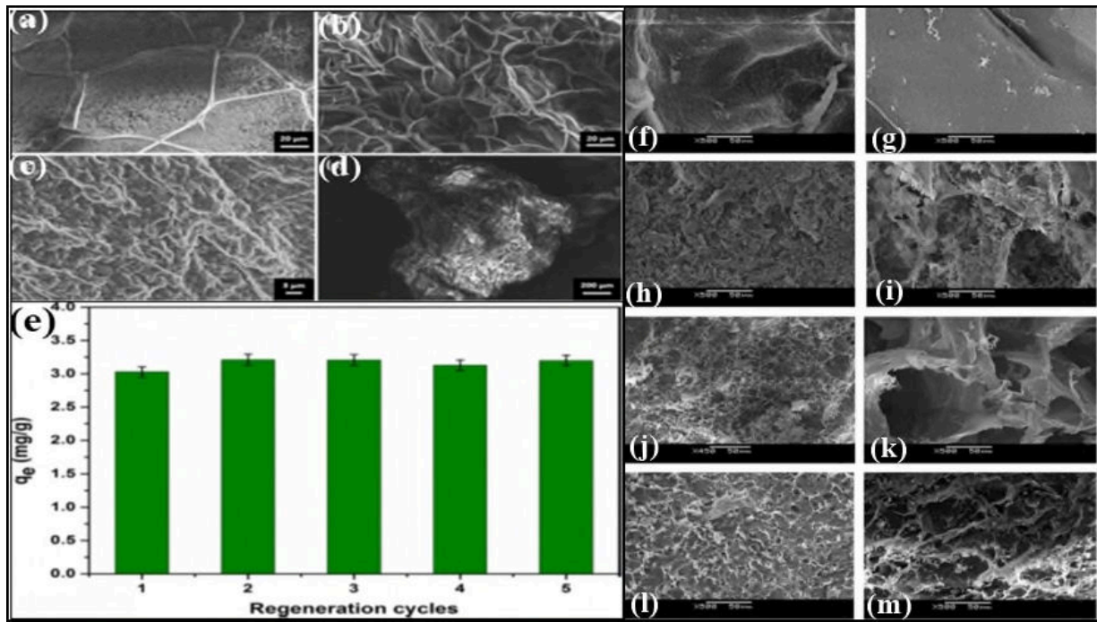
Figure 7. SEM images of (a) sodium alginate, (b) cellulose/sodium alginate hydrogel, (c) crosslinking behaviour of cellulose/sodium alginate hydrogel and (d) porous behaviour of cellulose/sodium alginate hydrogen [129]. Reprinted with permission from [129]. Copyright 2015 Springer, (e) reusability of the cellulose/sodium alginate hydrogel [129]. Reprinted with permission from [129]. Copyright 2015 Springer, SEM images of (f, g) pure cellulose hydrogel beads, (h, i) cellulose based collagen hydrogel beads (cellulose & collagen is 1:1), (j, k) prepared hydrogel (cellulose & collagen is 1:2), (l, m) prepared hydrogel (cellulose & collagen is 1:3) [141]. Reprinted with permission from [141]. Copyright 2013 Elsevier.
