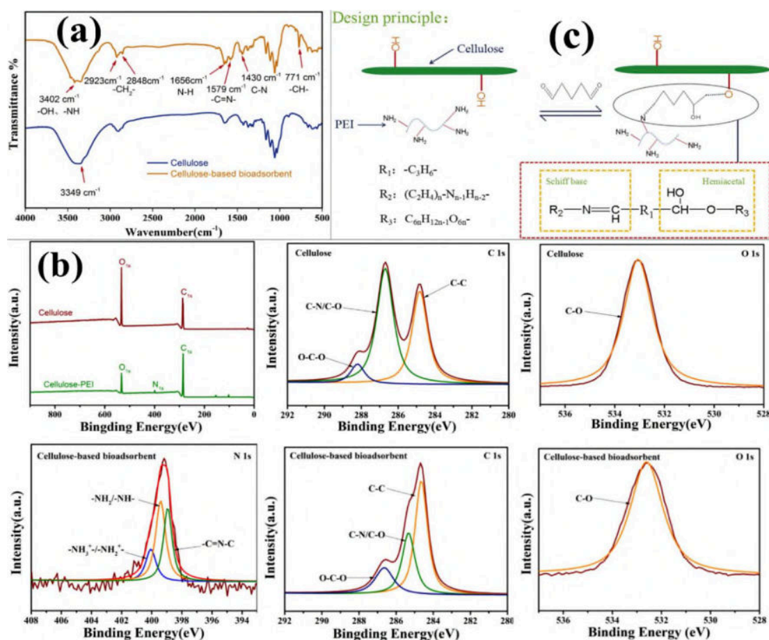
Figure 5. (a) FTIR spectra of pure cellulose and prepared bio-adsorbent [124]. Reprinted with permission from [124]. Copyright 2018 Elsevier, (b) XPS spectrum of pure cellulose and prepared bio-adsorbent [124]. Reprinted with permission from [124]. Copyright 2018 Elsevier, (c) proposed mechanism for the synthesis of bio-adsorbent [124]. Reprinted with permission from [124]. Copyright 2018 Elsevier.
