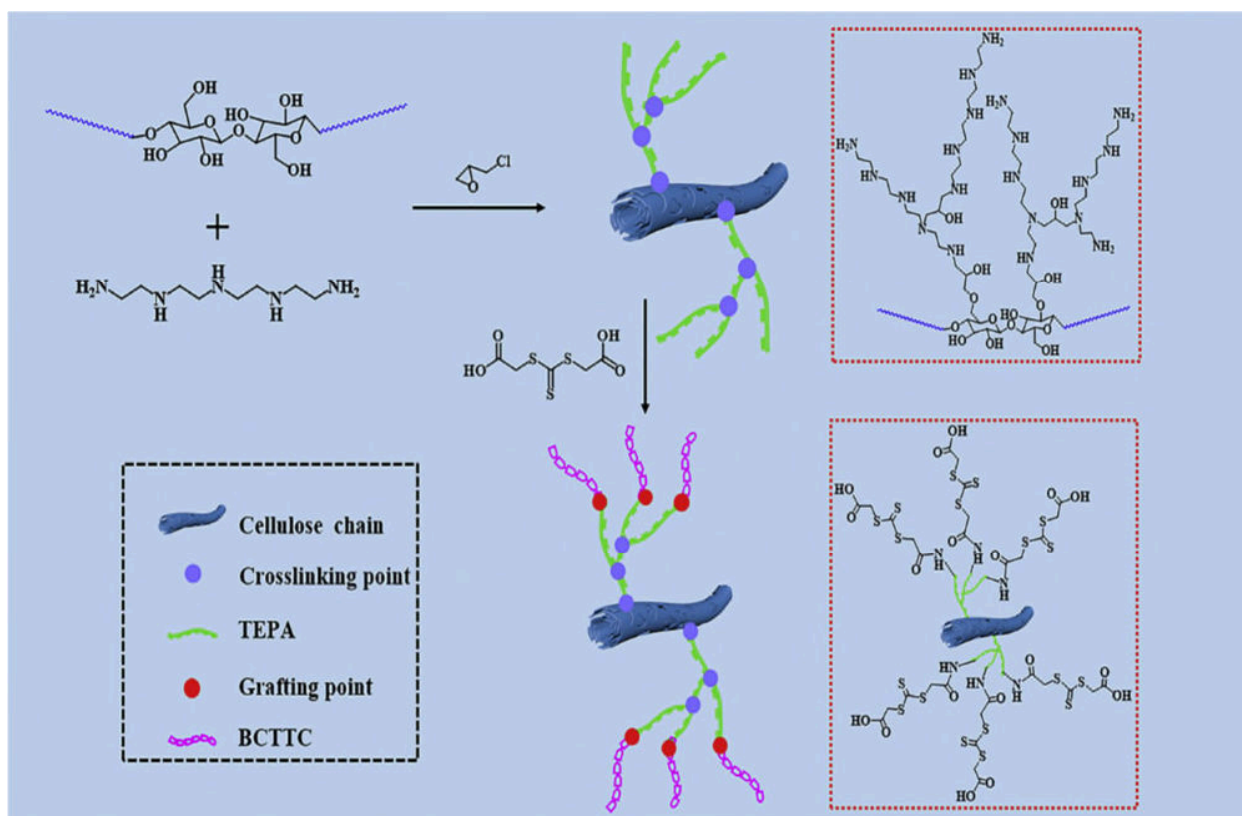
Figure 14. Figure shows the synthesis of cellulose-based adsorbent [135]. Reprinted with permission from [135]. Copyright 2020 Elsevier.
