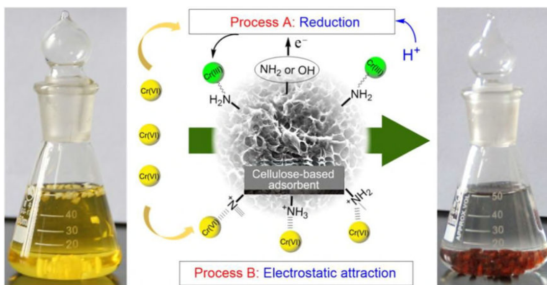
Figure 12. Proposed adsorption mechanism for Cr(VI) by synthesised adsorbent [133].
