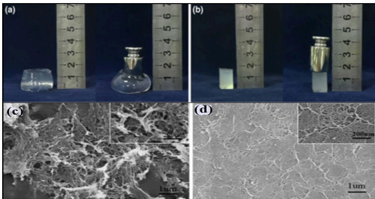
Figure 10. Representation of mechanical property of (a) cellulose based hydrogel (2 wt%) and (b) cellulose-based polyethylene imine hydrogel composite (cellulose 2 wt % and polyethylene imine 5 wt %) [140]. Reprinted with permission from [140]. Copyright 2016 Springer, SEM images of
