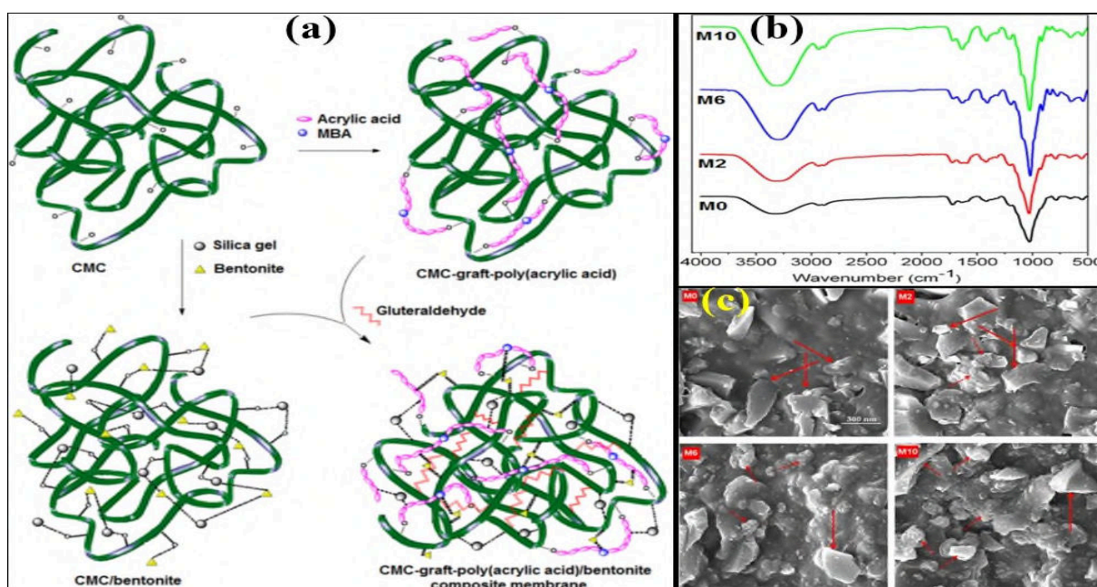
Figure 16. (a) Schematic representation for fabrication of carboxymethyl cellulose based poly (acrylic acid)/bentonite composite membrane [131]. Reprinted with permission from [131]. Copyright 2016 Elsevier, (b) FTIR spectrum of prepared grafted nanocomposite membranes. M0 (bentonite = 0), M2 (bentonite = 0.02 gm), M6 (bentonite = 0.06 gm) and M10 bentonite = 0.1 gm) [131]. Reprinted with permission from [131]. Copyright 2016 Elsevier, (c) SEM images of prepared nanocomposite membranes M0 (bentonite = 0), M2 (bentonite = 0.02 gm), M6 (bentonite = 0.06 gm) and M10 bentonite = 0.1 gm) [131]. Reprinted with permission from [131]. Copyright 2016 Elsevier.
