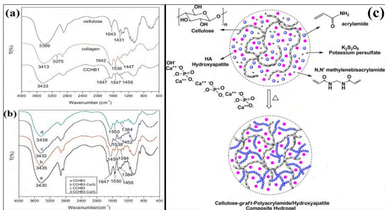
Figure 8. FTIR spectrum of (a) cellulose, collagen and cellulose-based collagen (cellulose & collagen is 1:1) hydrogel beads, (b) cellulose-based collagen (1:2) hydrogel beads (CCHB2), cellulose-based collagen (1:3) hydrogel beads (CCHB3) and Cu (II) ion adsorbed hydrogel beads [141]. Reprinted with permission from [141]. Copyright 2013 Elsevier, (c) possible mechanism for preparation of cellulose grafted polyacrylamide/hydroxyapatite hydrogel composite [142]. Reprinted with permission from [142]. Copyright 2013 Elsevier.
