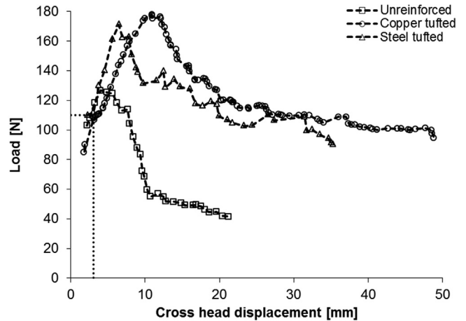
Fig. 3. Representative load-displacement curve of bindered composites tufted with copper and stainless steel.
