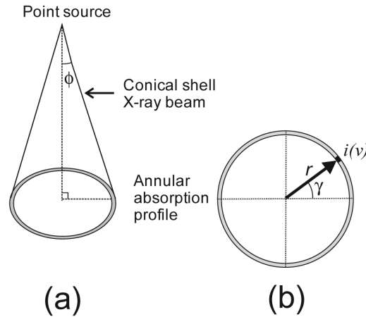
Fig. 2. (a) Conical shell interrogating beam with a half-opening angle of \phi . (b) Discretised ring sample v with intensity i at polar coordinate (r, \gamma) where the pole is the piercing point of the symmetry axis on the detector plane.
