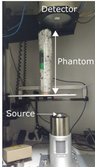
Fig. 9. Cylindrical phantom mounted on the translation table in the X-ray inspection system. An aggregate of discrete objects arranged along a \sim 38 cm component of the z-axis were supported by polystyrene foam.
