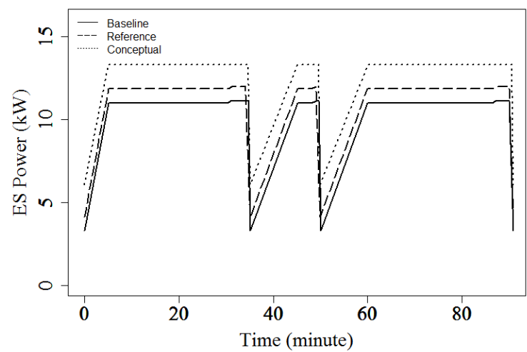
Fig. 5 Electrical System power demand
