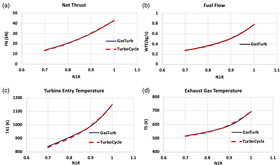
Figure 7. Comparison of steady state performance between TurboCycle and GasTurb models (a)–(d).
