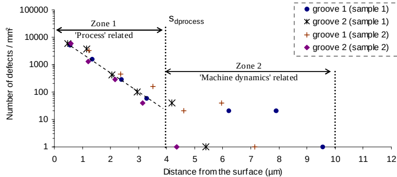
Fig. 7. ‘Process’ related and ‘Machine dynamics’ related zones (finish cut - D25) – a) ULE ® b) Zerodur ®
