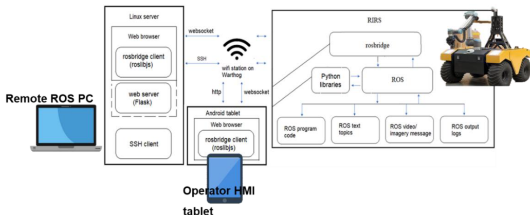
Fig. 14. Remote C&C subsystem structure.
