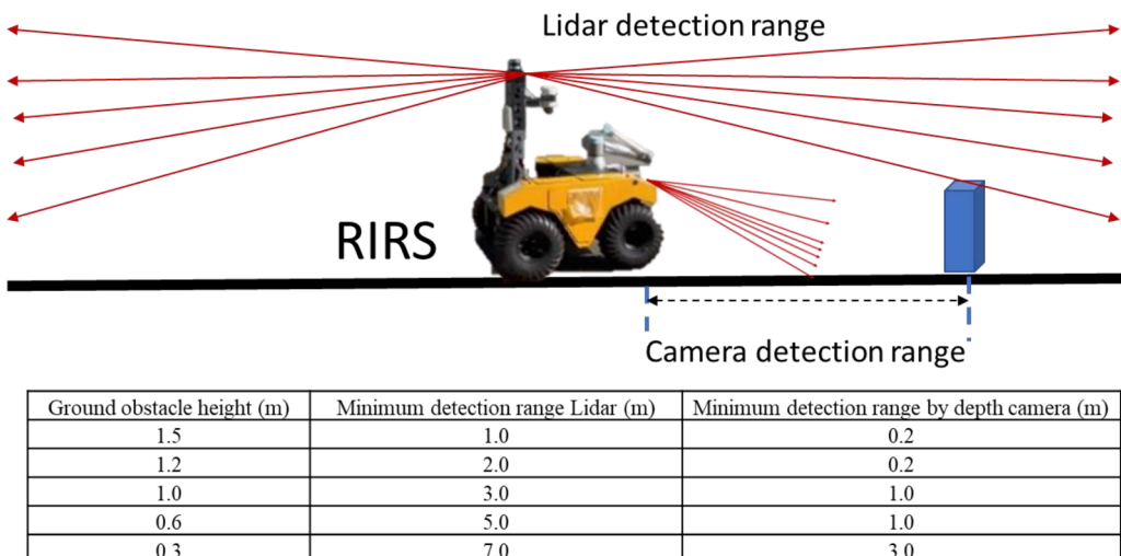
Fig. 25. Collision avoidance detection range calibration.
