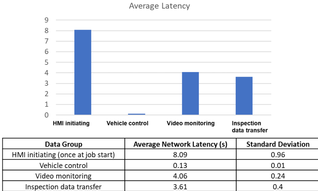
Fig. 24. The latency of different types of commands & data.
