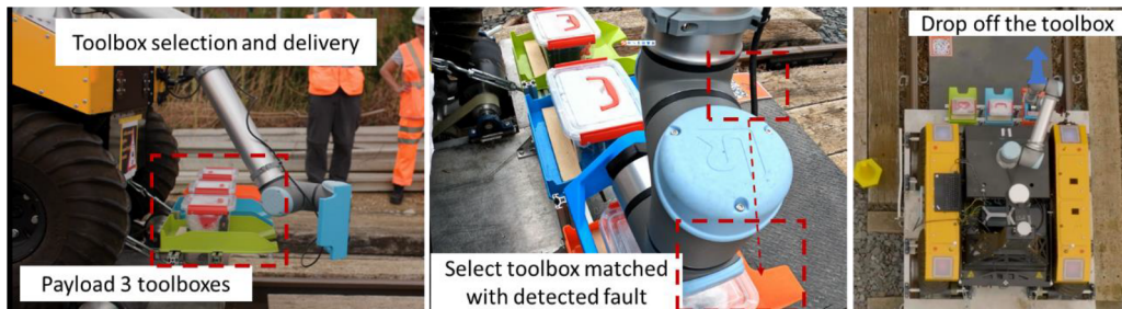
Fig. 21. The demonstration of Toolbox delivery testing.
