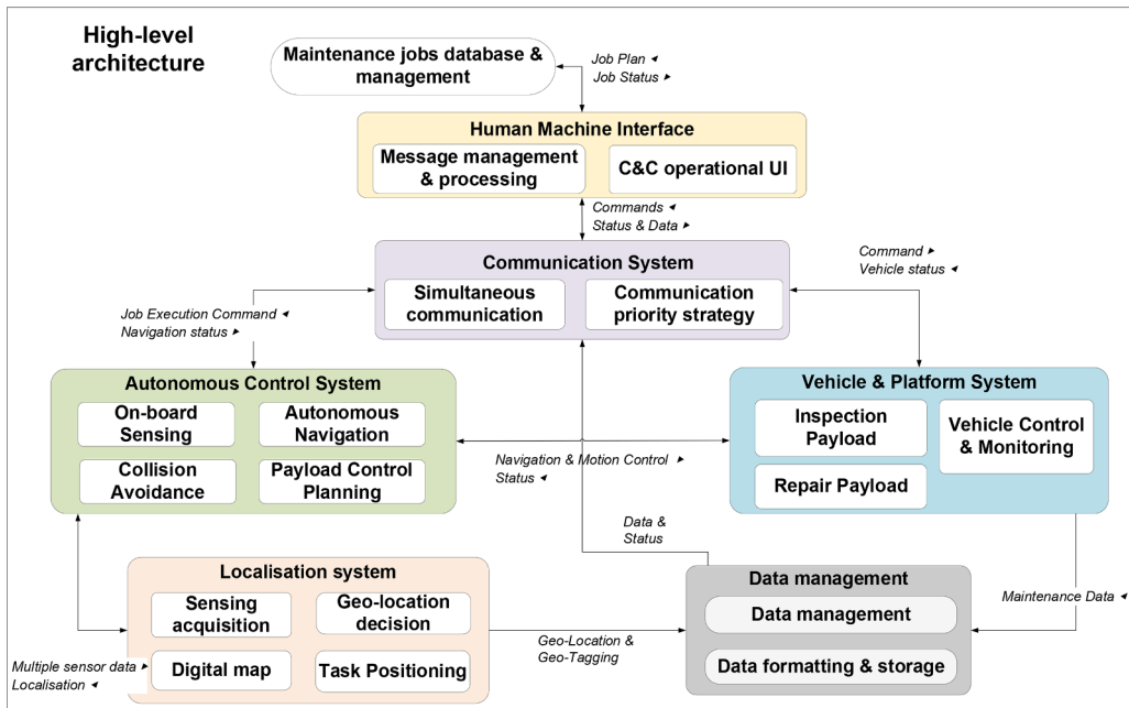
Fig. 5. The high-level architecture design of C&amp;C.
