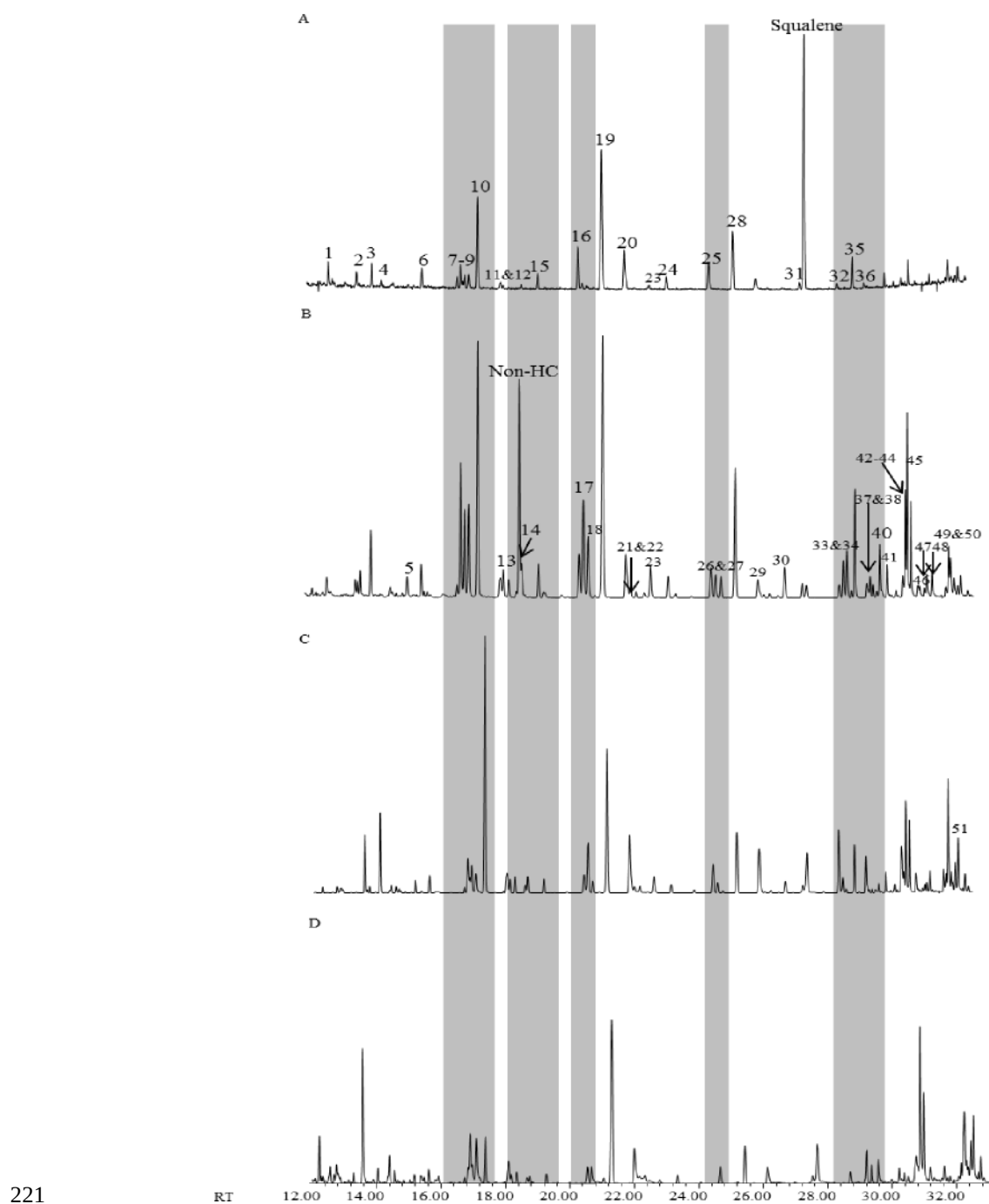
Figure 2. GC chromatograms of C. vomitoria larvae at four different ages, A: Day 1, B: Day 4, C: Day 8 and D: Day 13. Shaded bars illustrate distinctive changes over time indicating specific areas of interest
