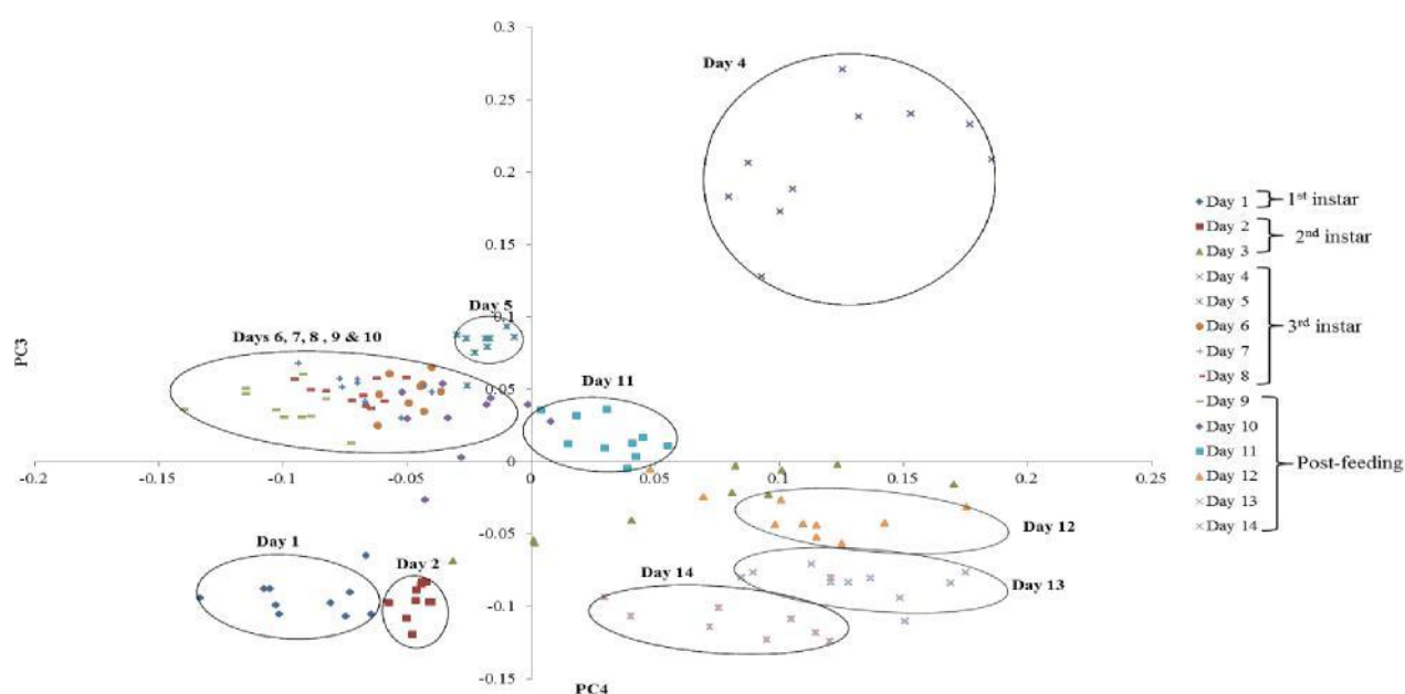
Figure 4: PCA plot showing PC4 against PC3 for C. vomitoria larvae using methyl branched alkanes only, with clustering days circled to catch the majority of that days points.
